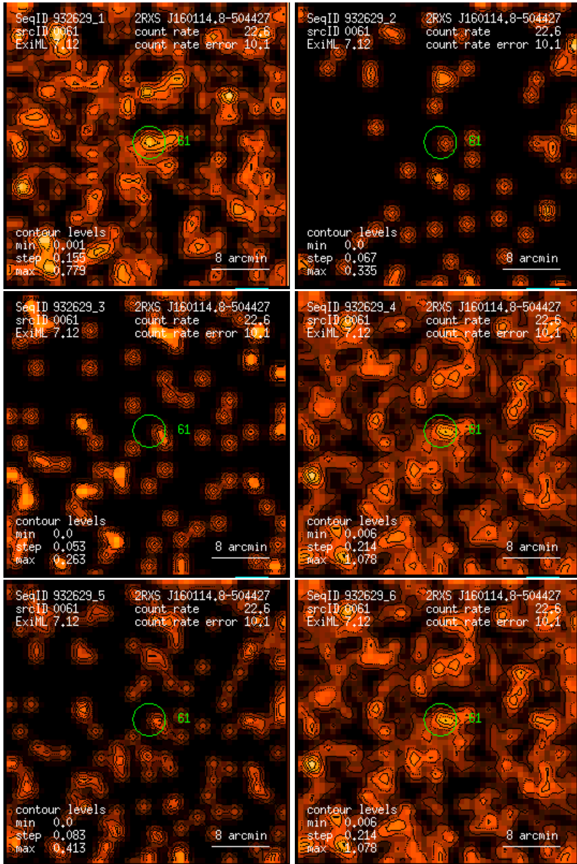
Figure 61: RASS 932629: detection 0061: band rate images, Gaussian filter: (1) PSPC channels 11 – 41, (2) 52 – 90, (3) 91 – 201, (4) 11 – 235, (5) 52 – 201, (6) 11 – 201. Broad band rates in counts/ks. Band rate contour levels in counts/ks/arcmin 2 .
