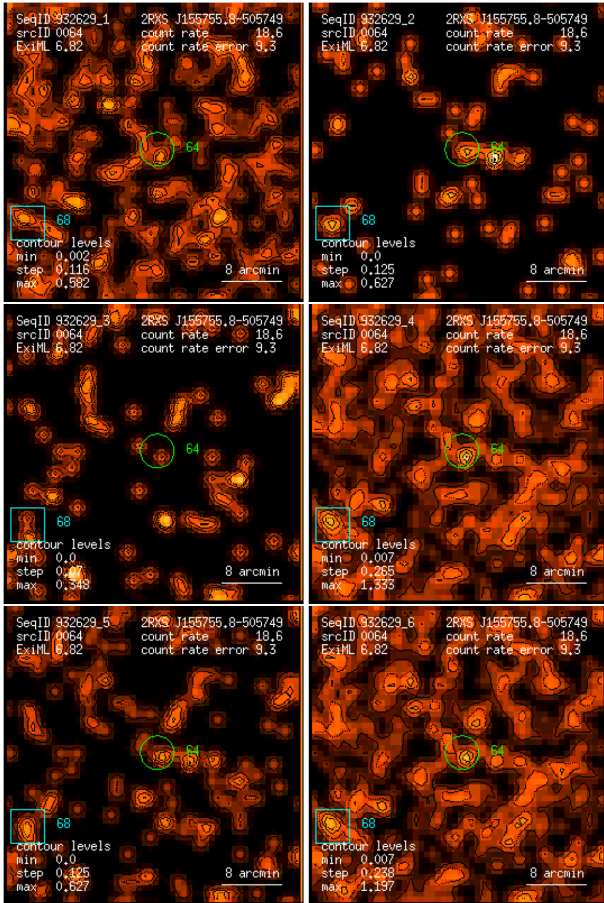
Figure 64: RASS 932629: detection 0064: band rate images, Gaussian filter: (1) PSPC channels 11 – 41, (2) 52 – 90, (3) 91 – 201, (4) 11 – 235, (5) 52 – 201, (6) 11 – 201. Broad band rates in counts/ks. Band rate contour levels in counts/ks/arcmin 2 .
