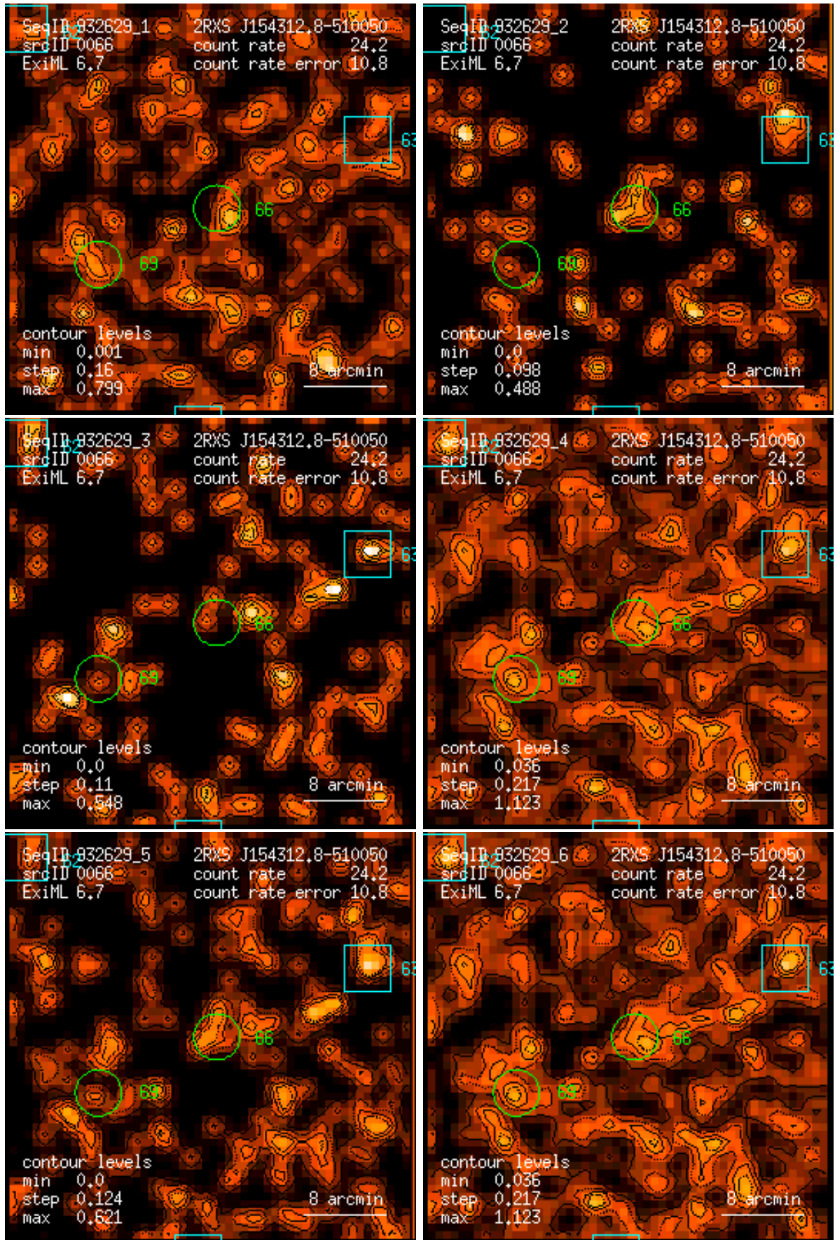
Figure 66: RASS 932629: detection 0066: band rate images, Gaussian filter: (1) PSPC channels 11 – 41, (2) 52 – 90, (3) 91 – 201, (4) 11 – 235, (5) 52 – 201, (6) 11 – 201. Broad band rates in counts/ks. Band rate contour levels in counts/ks/arcmin 2 .
