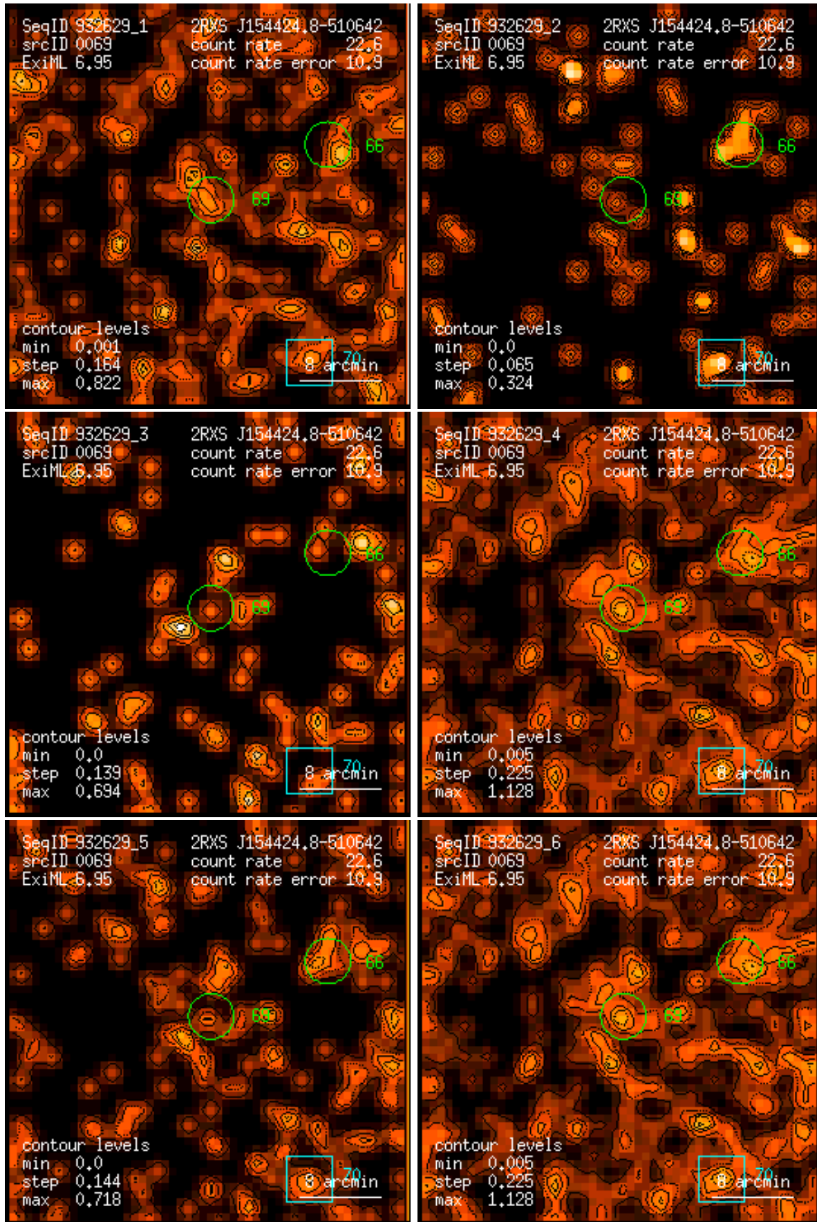
Figure 69: RASS 932629: detection 0069: band rate images, Gaussian filter: (1) PSPC channels 11 – 41, (2) 52 – 90, (3) 91 – 201, (4) 11 – 235, (5) 52 – 201, (6) 11 – 201. Broad band rates in counts/ks. Band rate contour levels in counts/ks/arcmin 2 .
