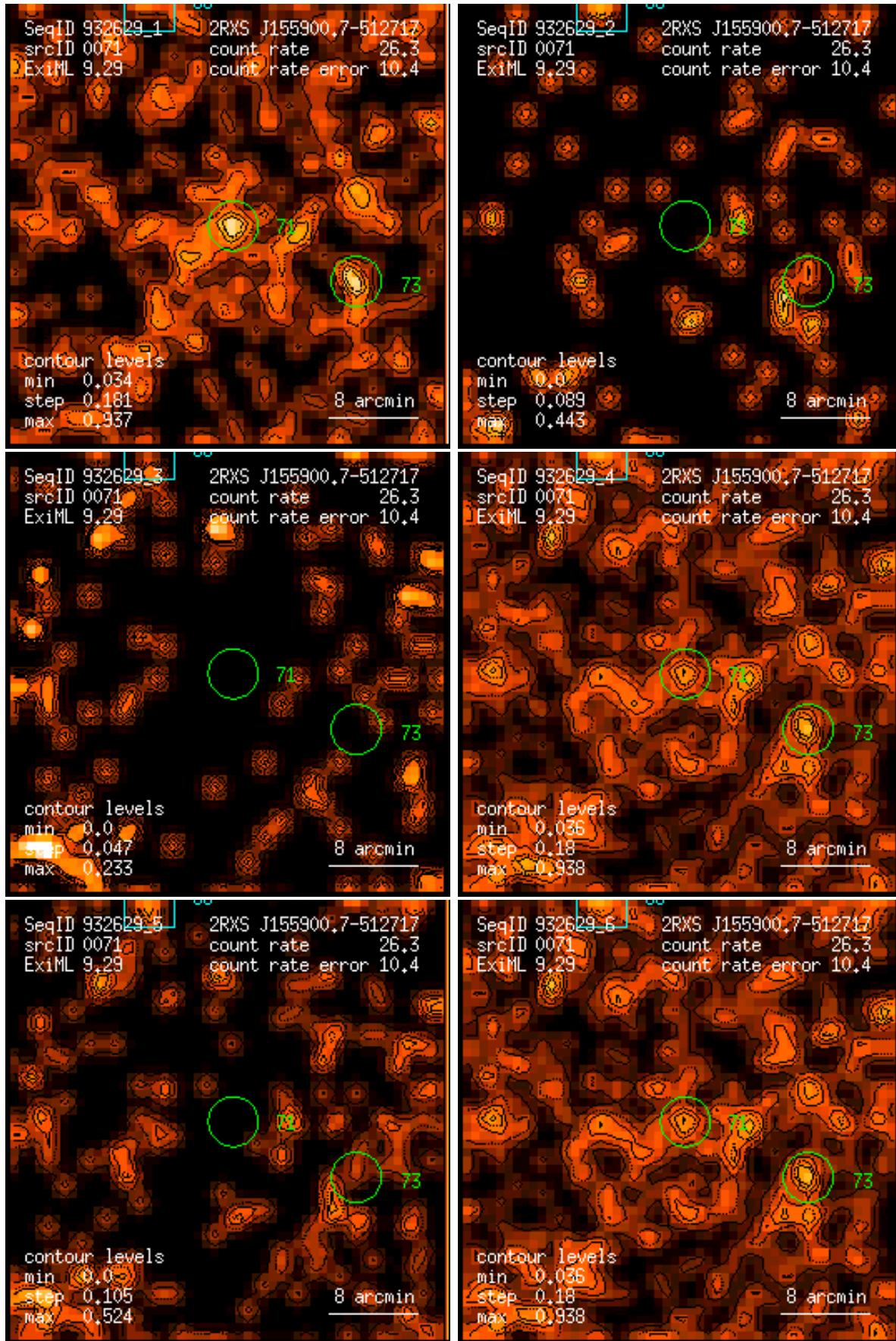
Figure 71: RASS 932629: detection 0071: band rate images, Gaussian filter: (1) PSPC channels 11 – 41, (2) 52 – 90, (3) 91 – 201, (4) 11 – 235, (5) 52 – 201, (6) 11 – 201. Broad band rates in counts/ks. Band rate contour levels in counts/ks/arcmin 2 .
