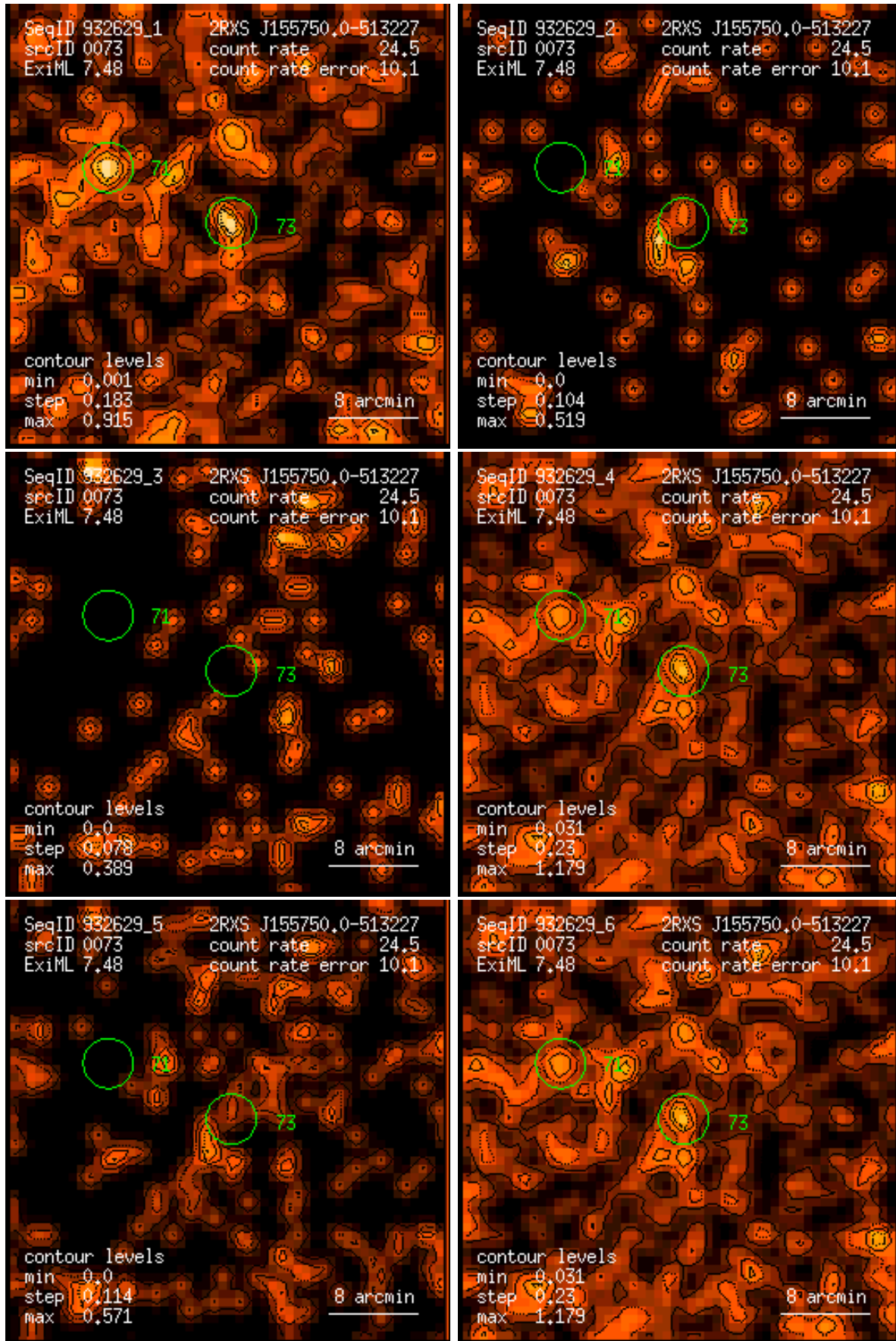
Figure 73: RASS 932629: detection 0073: band rate images, Gaussian filter: (1) PSPC channels 11 – 41, (2) 52 – 90, (3) 91 – 201, (4) 11 – 235, (5) 52 – 201, (6) 11 – 201. Broad band rates in counts/ks. Band rate contour levels in counts/ks/arcmin 2 .
