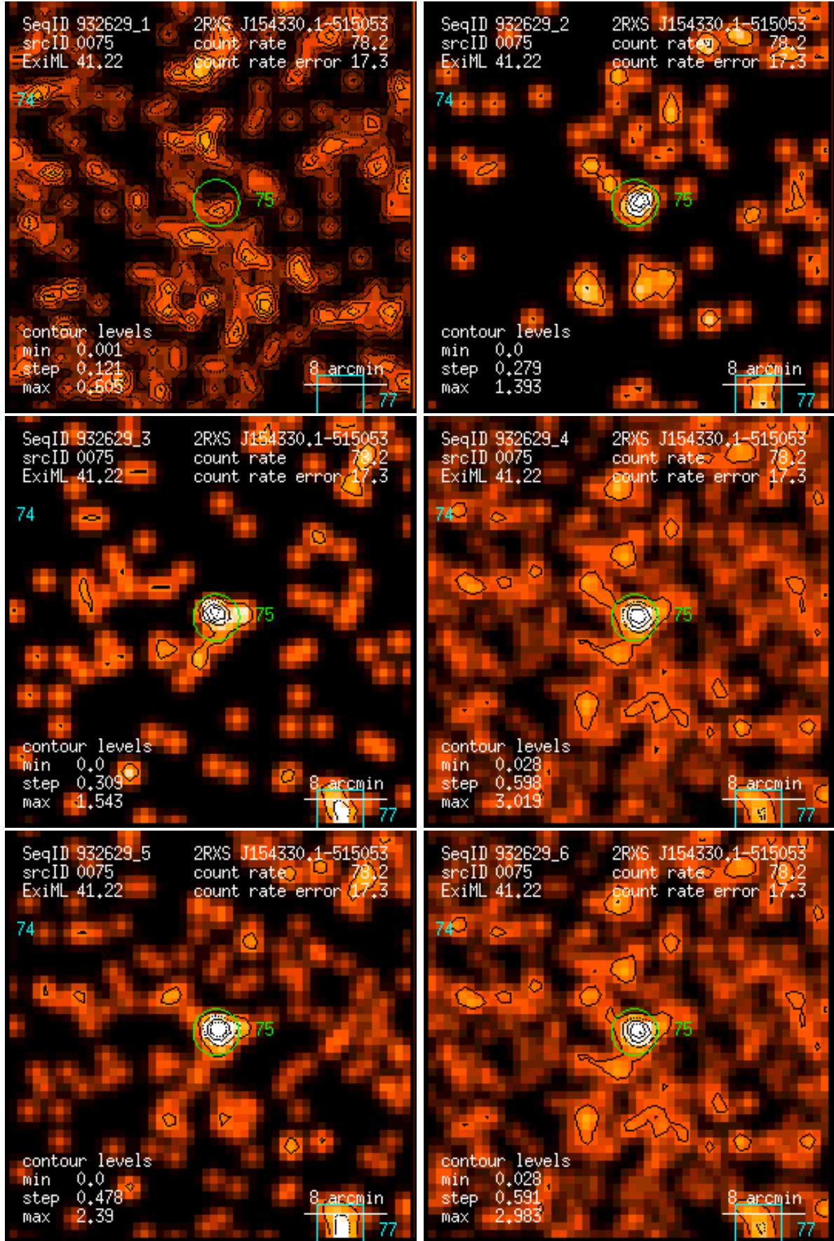
Figure 75: RASS 932629: detection 0075: band rate images, Gaussian filter: (1) PSPC channels 11 – 41, (2) 52 – 90, (3) 91 – 201, (4) 11 – 235, (5) 52 – 201, (6) 11 – 201. Broad band rates in counts/ks. Band rate contour levels in counts/ks/arcmin 2 .
