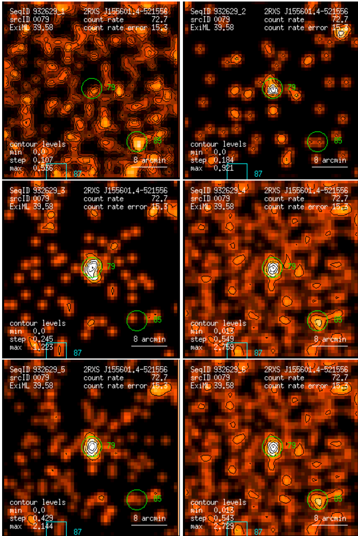
Figure 79: RASS 932629: detection 0079: band rate images, Gaussian filter: (1) PSPC channels 11 – 41, (2) 52 – 90, (3) 91 – 201, (4) 11 – 235, (5) 52 – 201, (6) 11 – 201. Broad band rates in counts/ks. Band rate contour levels in counts/ks/arcmin 2 .
