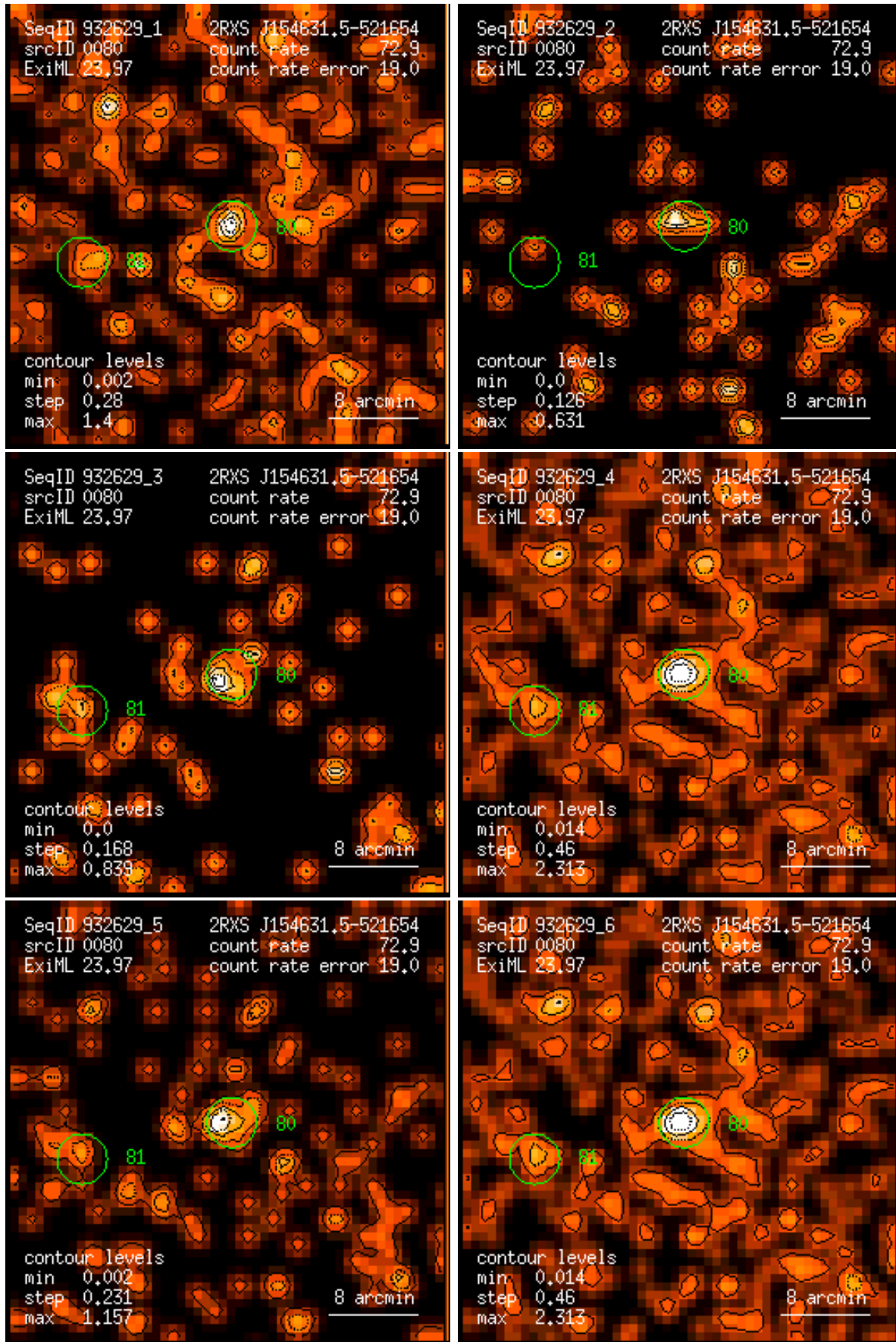
Figure 80: RASS 932629: detection 0080: band rate images, Gaussian filter: (1) PSPC channels 11 – 41, (2) 52 – 90, (3) 91 – 201, (4) 11 – 235, (5) 52 – 201, (6) 11 – 201. Broad band rates in counts/ks. Band rate contour levels in counts/ks/arcmin 2 .
