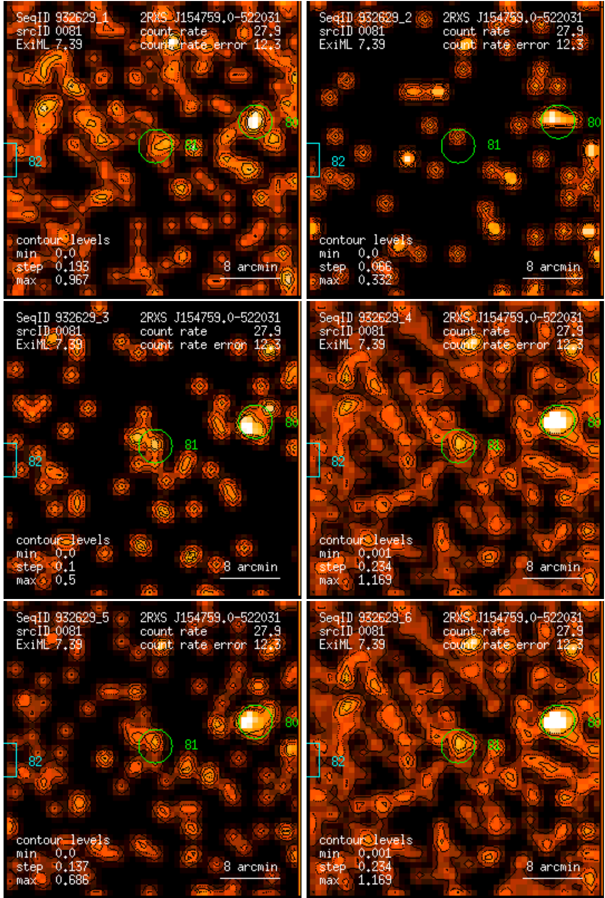
Figure 81: RASS 932629: detection 0081: band rate images, Gaussian filter: (1) PSPC channels 11 – 41, (2) 52 – 90, (3) 91 – 201, (4) 11 – 235, (5) 52 – 201, (6) 11 – 201. Broad band rates in counts/ks. Band rate contour levels in counts/ks/arcmin 2 .
