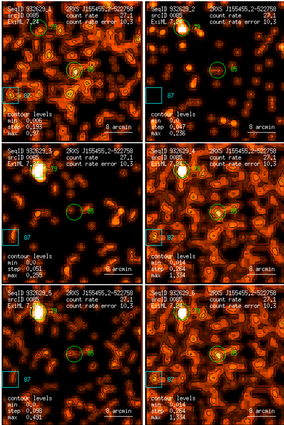
Figure 85: RASS 932629: detection 0085: band rate images, Gaussian filter: (1) PSPC channels 11 – 41, (2) 52 – 90, (3) 91 – 201, (4) 11 – 235, (5) 52 – 201, (6) 11 – 201. Broad band rates in counts/ks. Band rate contour levels in counts/ks/arcmin 2 .
