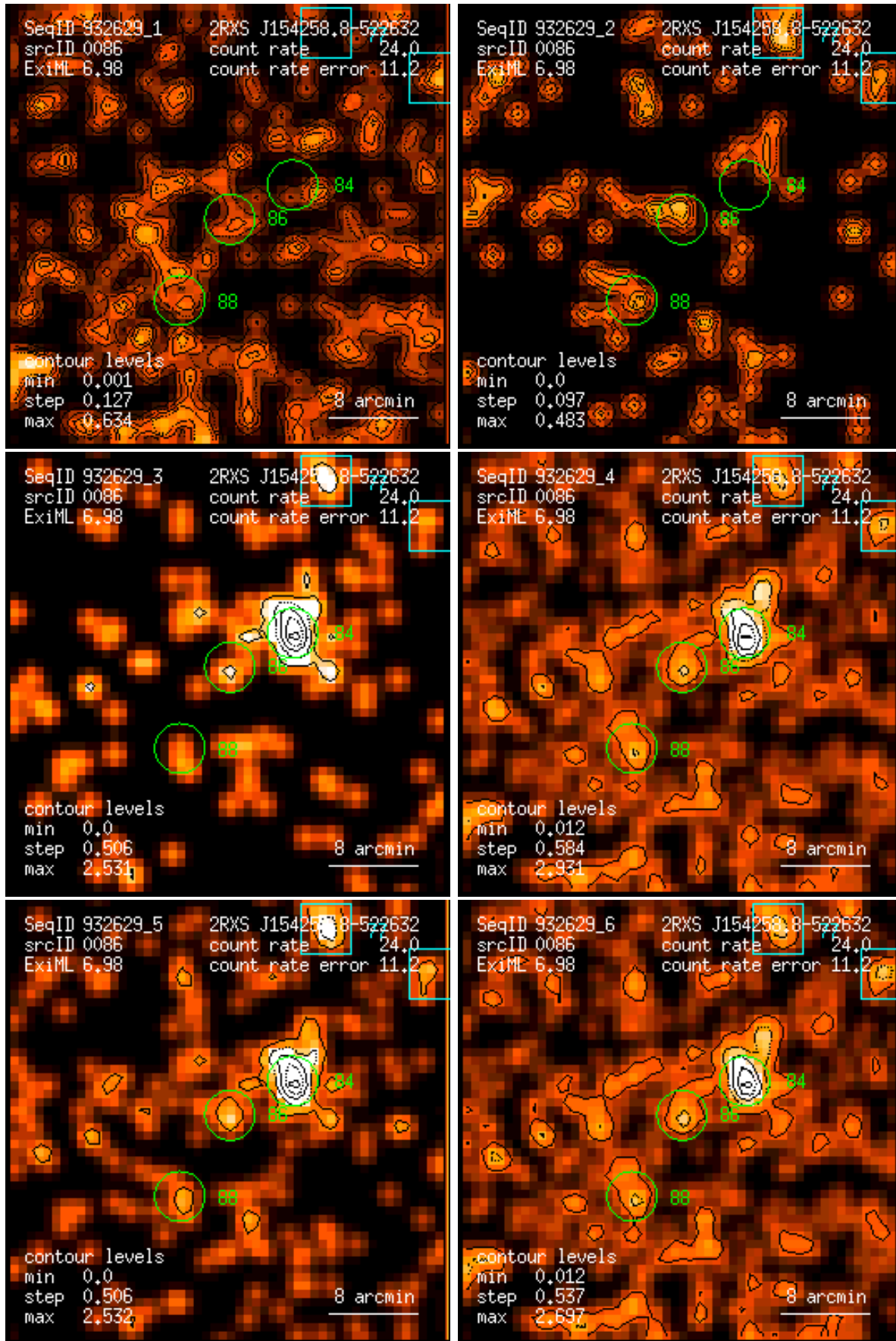
Figure 86: RASS 932629: detection 0086: band rate images, Gaussian filter: (1) PSPC channels 11 – 41, (2) 52 – 90, (3) 91 – 201, (4) 11 – 235, (5) 52 – 201, (6) 11 – 201. Broad band rates in counts/ks. Band rate contour levels in counts/ks/arcmin 2 .
