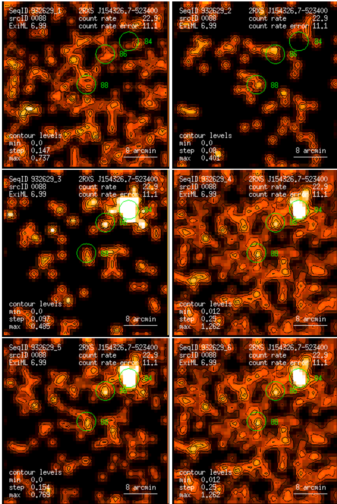
Figure 88: RASS 932629: detection 0088: band rate images, Gaussian filter: (1) PSPC channels 11 – 41, (2) 52 – 90, (3) 91 – 201, (4) 11 – 235, (5) 52 – 201, (6) 11 – 201. Broad band rates in counts/ks. Band rate contour levels in counts/ks/arcmin 2 .
