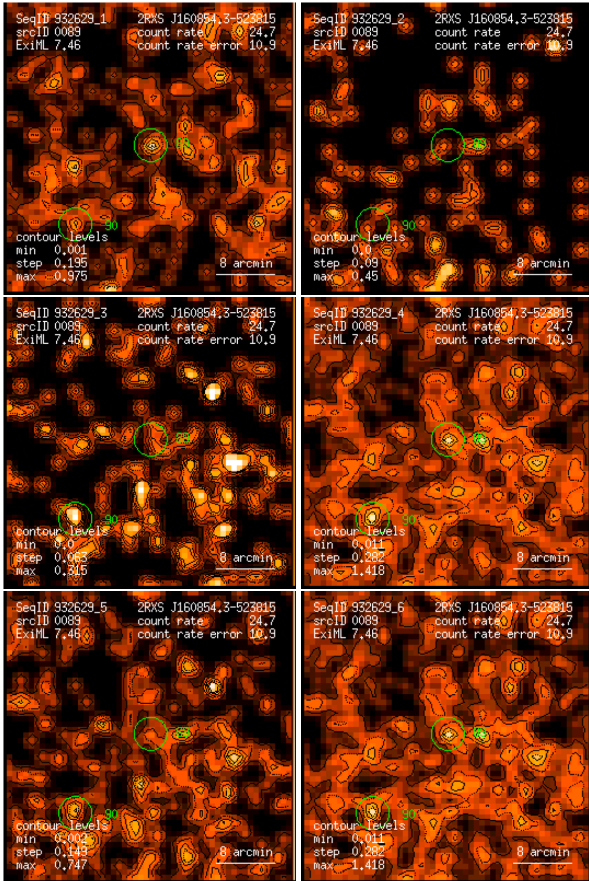
Figure 89: RASS 932629: detection 0089: band rate images, Gaussian filter: (1) PSPC channels 11 – 41, (2) 52 – 90, (3) 91 – 201, (4) 11 – 235, (5) 52 – 201, (6) 11 – 201. Broad band rates in counts/ks. Band rate contour levels in counts/ks/arcmin 2 .
