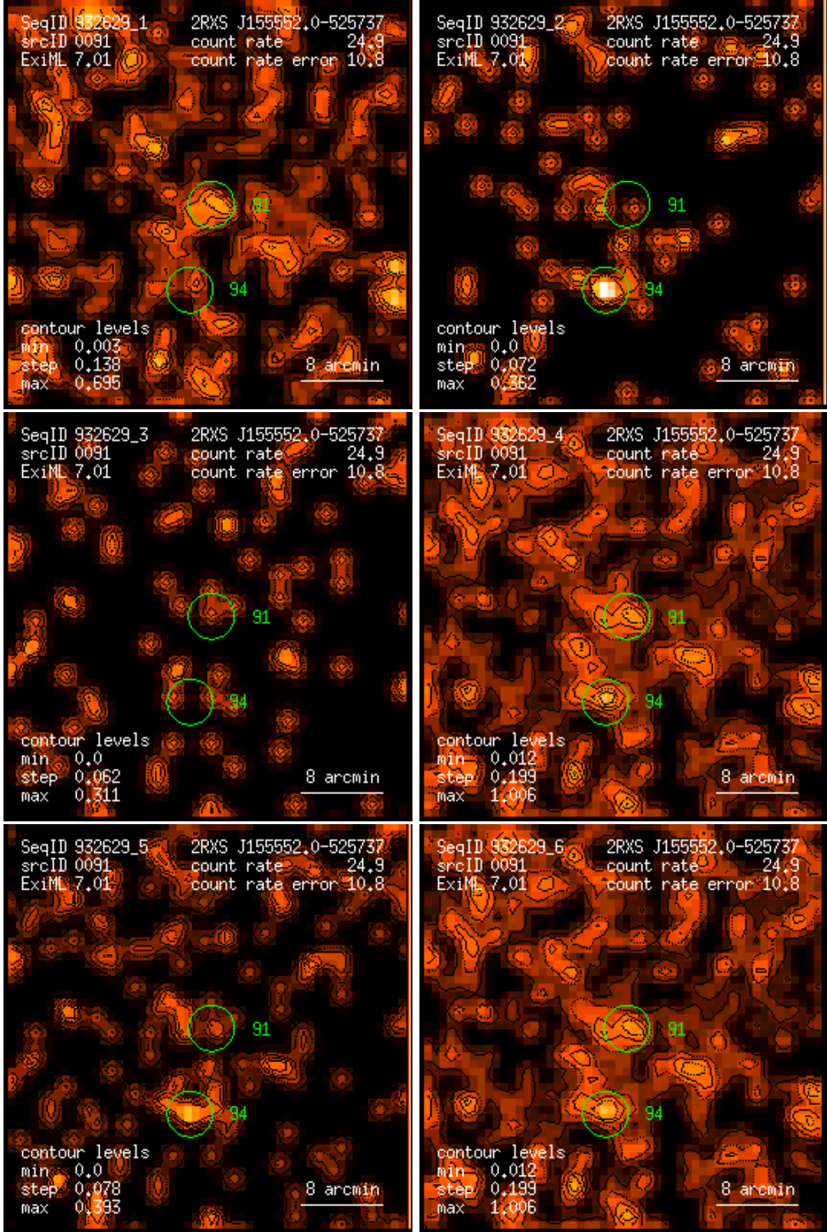
Figure 91: RASS 932629: detection 0091: band rate images, Gaussian filter: (1) PSPC channels 11 – 41, (2) 52 – 90, (3) 91 – 201, (4) 11 – 235, (5) 52 – 201, (6) 11 – 201. Broad band rates in counts/ks. Band rate contour levels in counts/ks/arcmin 2 .
