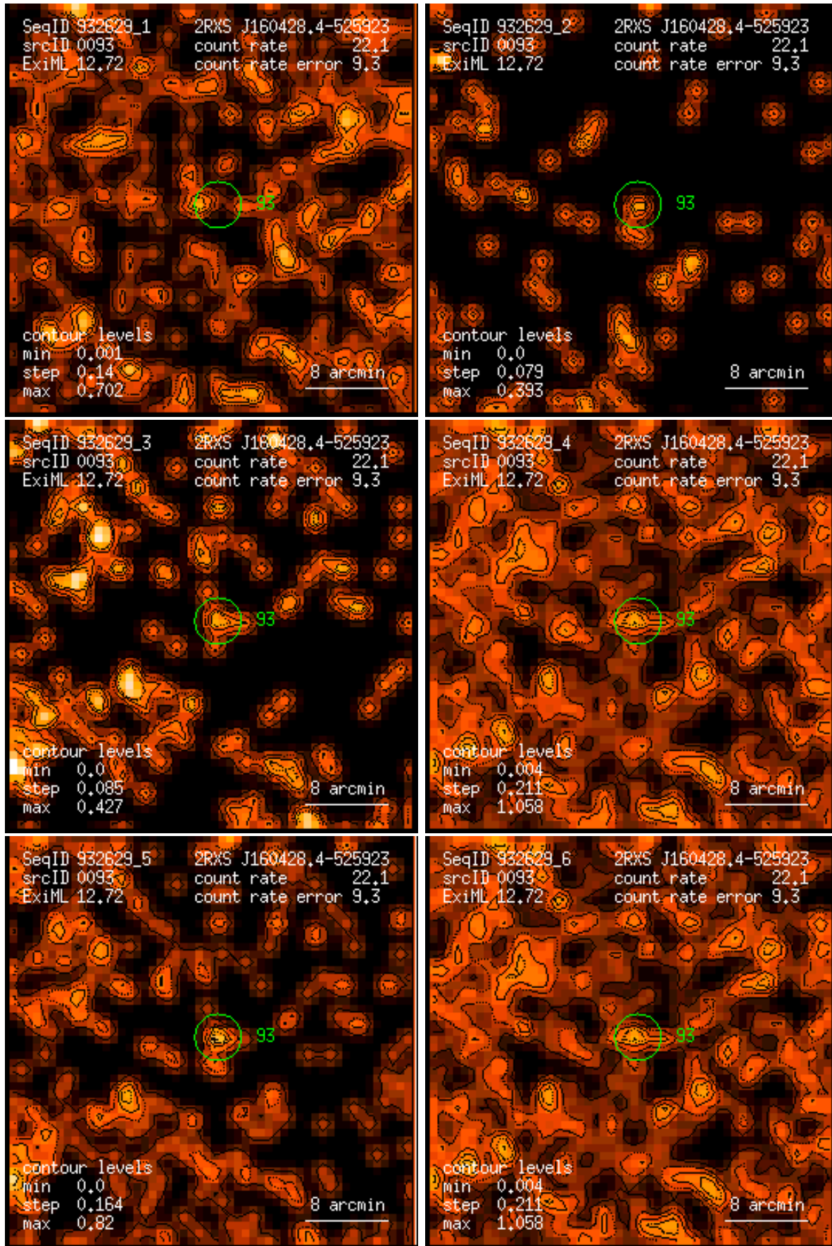
Figure 93: RASS 932629: detection 0093: band rate images, Gaussian filter: (1) PSPC channels 11 – 41, (2) 52 – 90, (3) 91 – 201, (4) 11 – 235, (5) 52 – 201, (6) 11 – 201. Broad band rates in counts/ks. Band rate contour levels in counts/ks/arcmin 2 .
