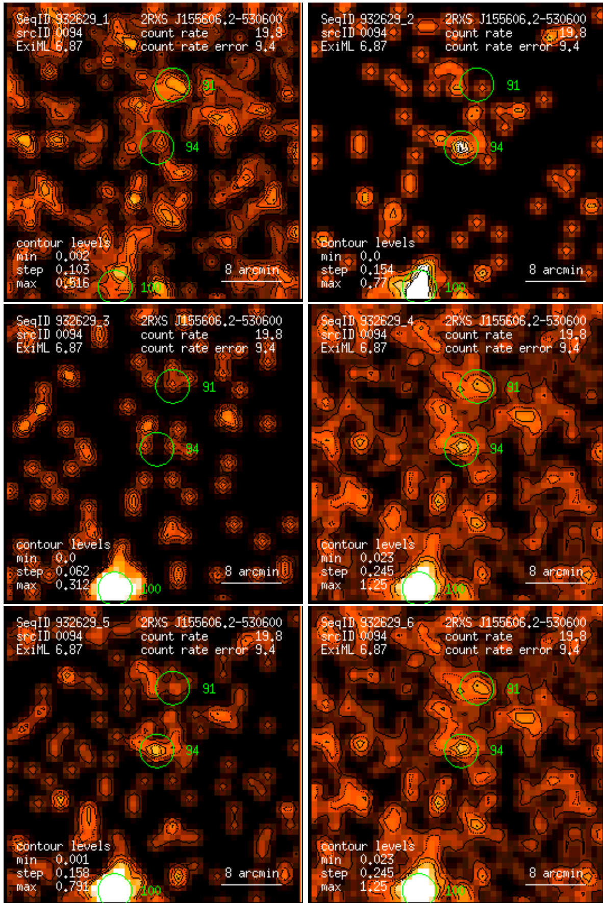
Figure 94: RASS 932629: detection 0094: band rate images, Gaussian filter: (1) PSPC channels 11 – 41, (2) 52 – 90, (3) 91 – 201, (4) 11 – 235, (5) 52 – 201, (6) 11 – 201. Broad band rates in counts/ks. Band rate contour levels in counts/ks/arcmin 2 .
