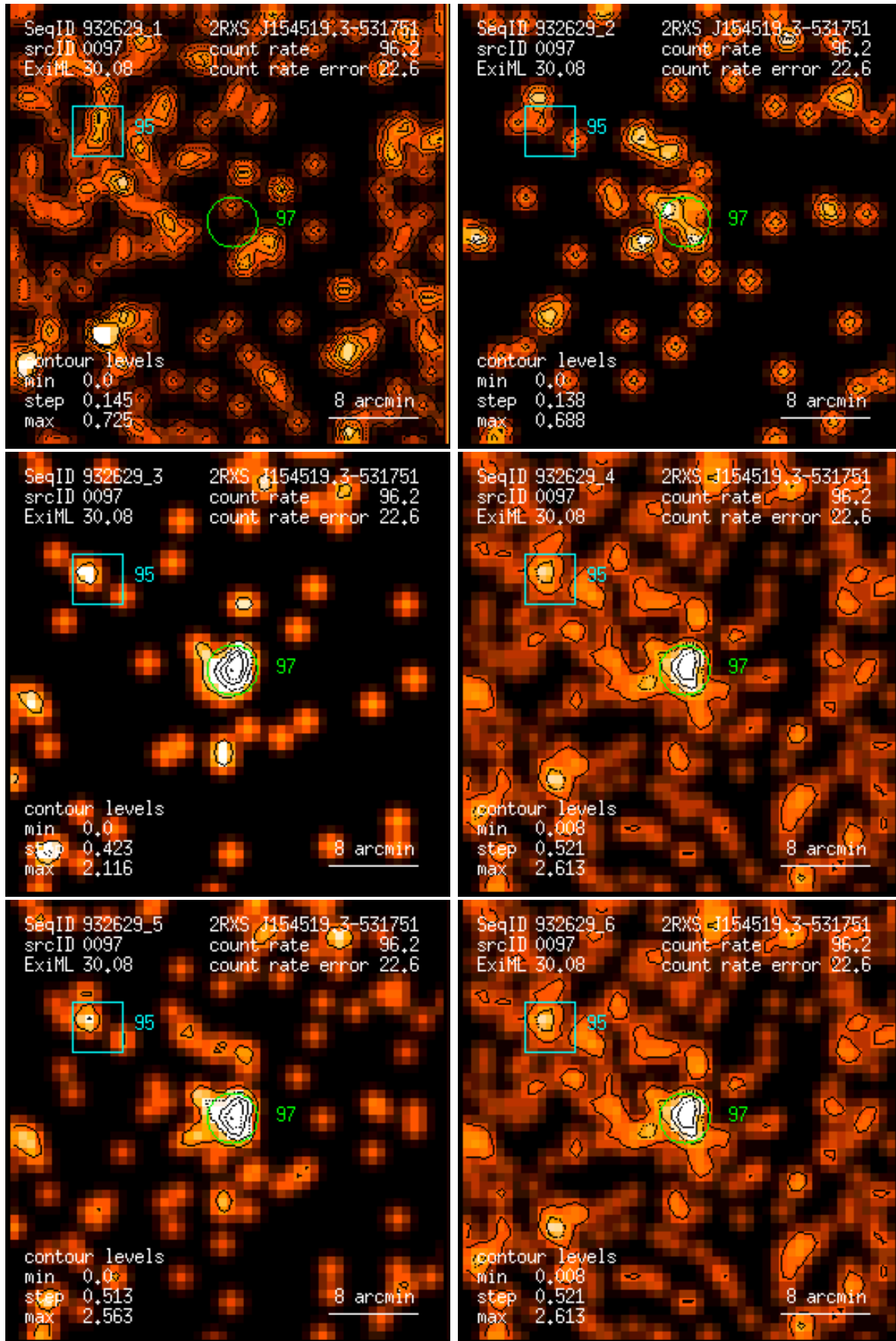
Figure 97: RASS 932629: detection 0097: band rate images, Gaussian filter: (1) PSPC channels 11 – 41, (2) 52 – 90, (3) 91 – 201, (4) 11 – 235, (5) 52 – 201, (6) 11 – 201. Broad band rates in counts/ks. Band rate contour levels in counts/ks/arcmin 2 .
