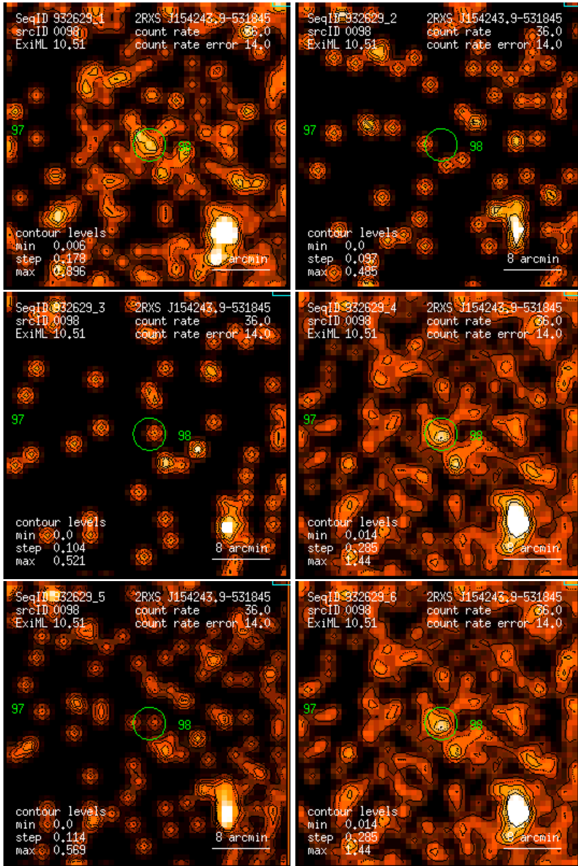
Figure 98: RASS 932629: detection 0098: band rate images, Gaussian filter: (1) PSPC channels 11 – 41, (2) 52 – 90, (3) 91 – 201, (4) 11 – 235, (5) 52 – 201, (6) 11 – 201. Broad band rates in counts/ks. Band rate contour levels in counts/ks/arcmin 2 .
