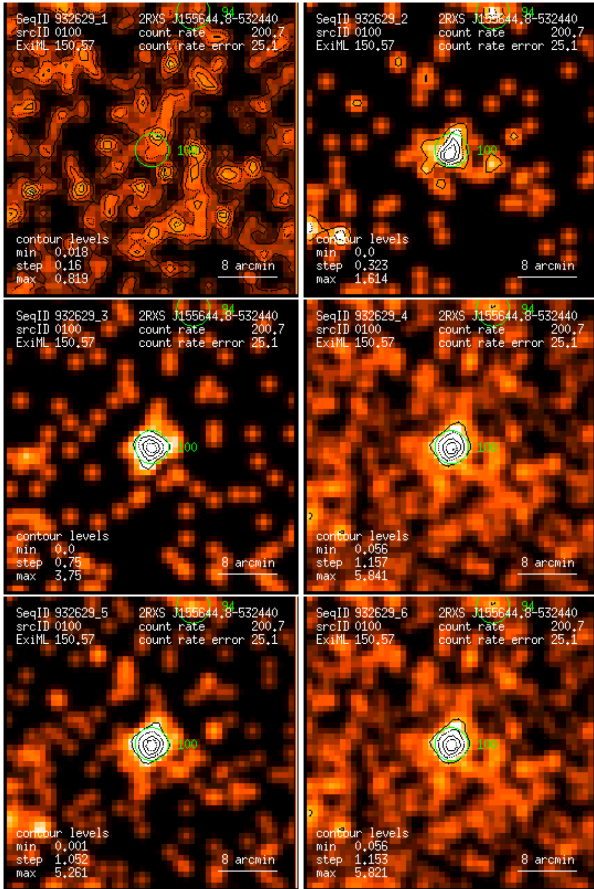
Figure 100: RASS 932629: detection 0100: band rate images, Gaussian filter: (1) PSPC channels 11 – 41, (2) 52 – 90, (3) 91 – 201, (4) 11 – 235, (5) 52 – 201, (6) 11 – 201. Broad band rates in counts/ks. Band rate contour levels in counts/ks/arcmin 2 .
