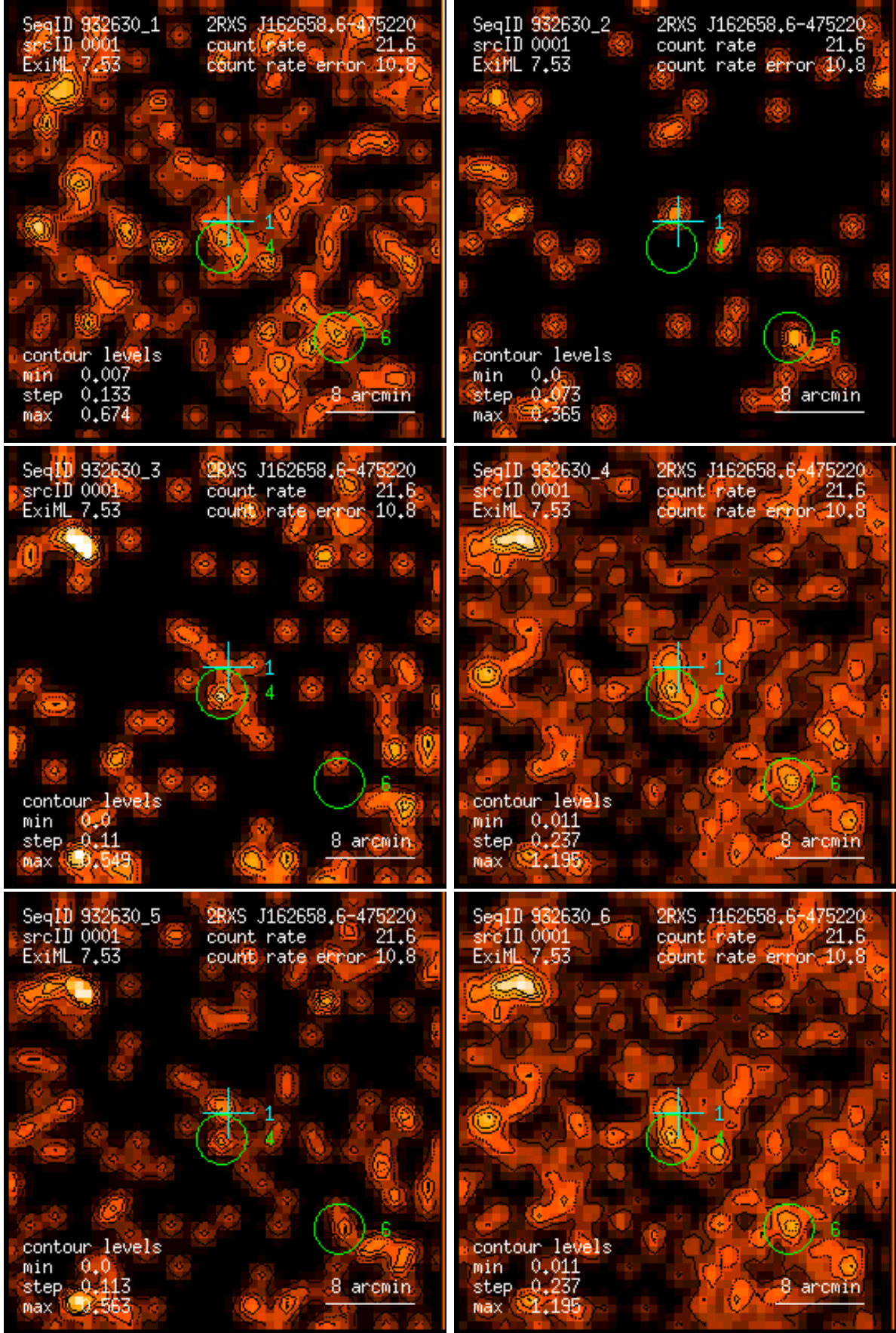
Figure 1: RASS 932630: detection 0001: band rate images, Gaussian filter: (1) PSPC channels 11 – 41, (2) 52 – 90, (3) 91 – 201, (4) 11 – 235, (5) 52 – 201, (6) 11 – 201. Broad band rates in counts/ks. Band rate contour levels in counts/ks/arcmin 2 .
