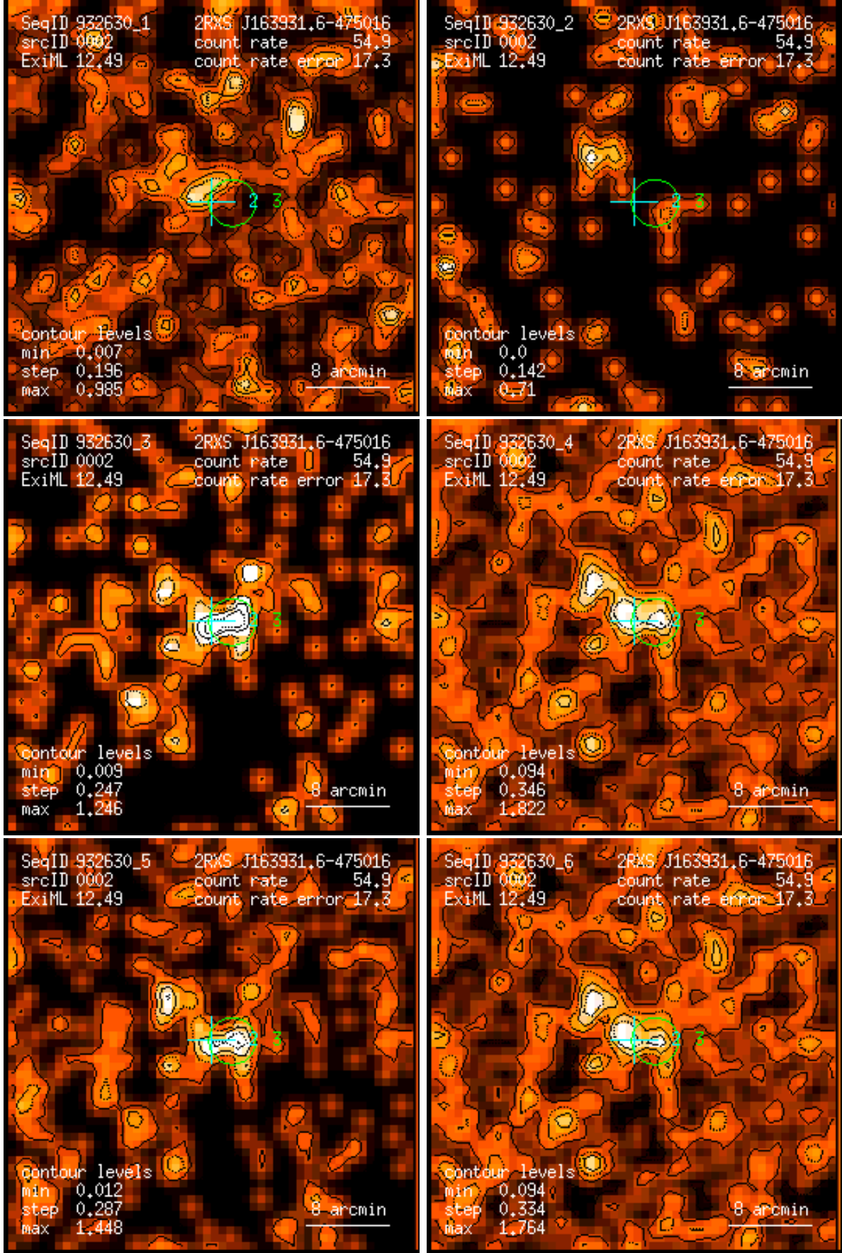
Figure 2: RASS 932630: detection 0002: band rate images, Gaussian filter: (1) PSPC channels 11 – 41, (2) 52 – 90, (3) 91 – 201, (4) 11 – 235, (5) 52 – 201, (6) 11 – 201. Broad band rates in counts/ks. Band rate contour levels in counts/ks/arcmin 2 .
