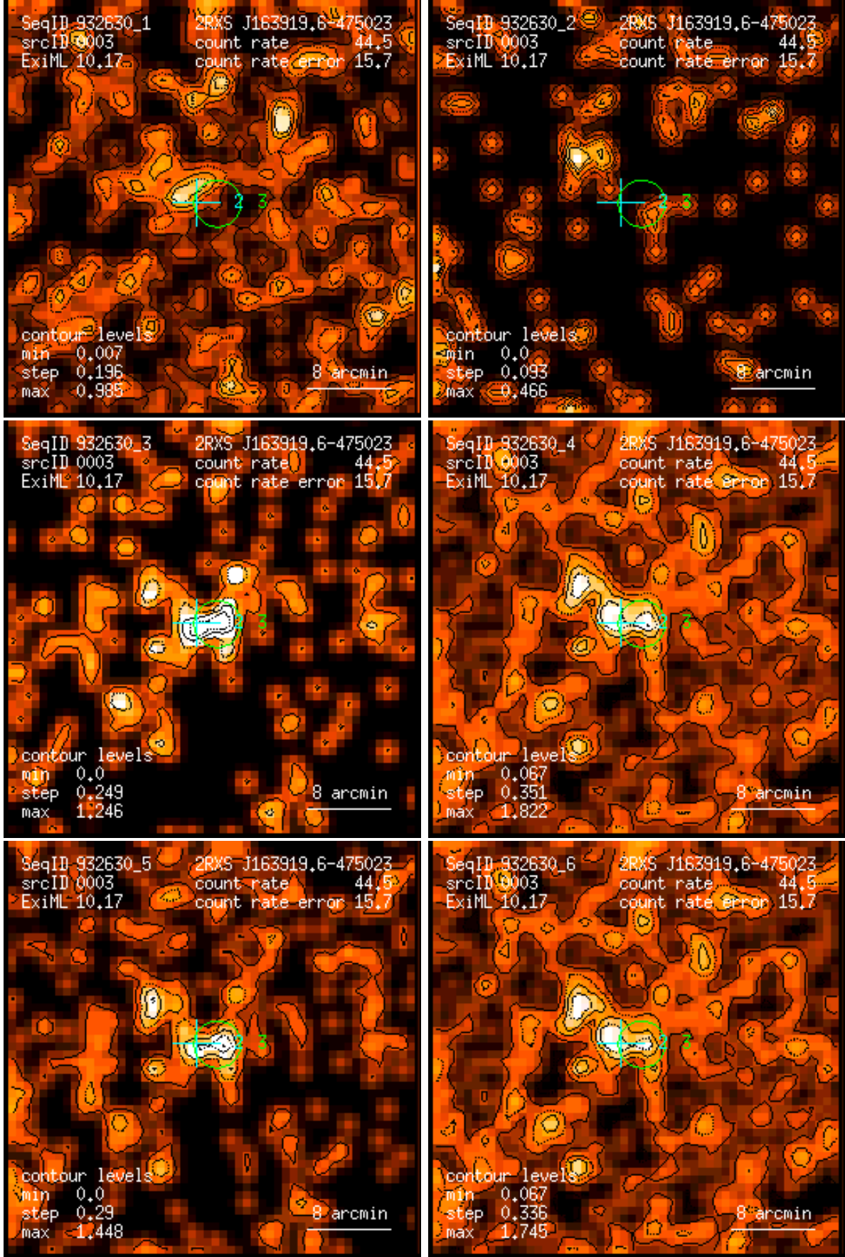
Figure 3: RASS 932630: detection 0003: band rate images, Gaussian filter: (1) PSPC channels 11 – 41, (2) 52 – 90, (3) 91 – 201, (4) 11 – 235, (5) 52 – 201, (6) 11 – 201. Broad band rates in counts/ks. Band rate contour levels in counts/ks/arcmin 2 .
