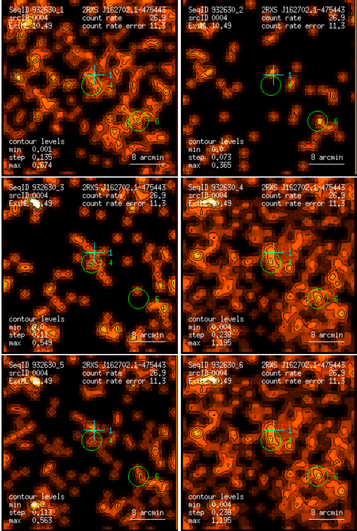
Figure 4: RASS 932630: detection 0004: band rate images, Gaussian filter: (1) PSPC channels 11 – 41, (2) 52 – 90, (3) 91 – 201, (4) 11 – 235, (5) 52 – 201, (6) 11 – 201. Broad band rates in counts/ks. Band rate contour levels in counts/ks/arcmin 2 .
