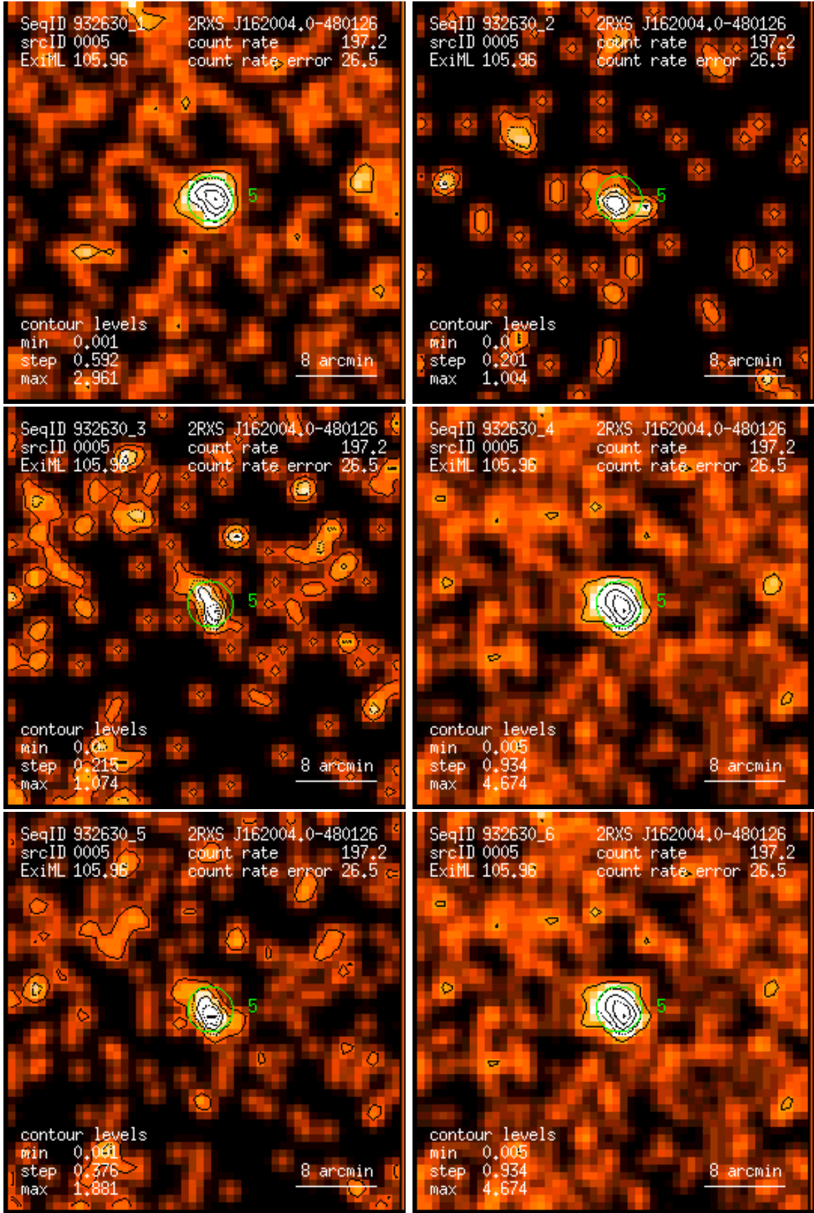
Figure 5: RASS 932630: detection 0005: band rate images, Gaussian filter: (1) PSPC channels 11 – 41, (2) 52 – 90, (3) 91 – 201, (4) 11 – 235, (5) 52 – 201, (6) 11 – 201. Broad band rates in counts/ks. Band rate contour levels in counts/ks/arcmin 2 .
