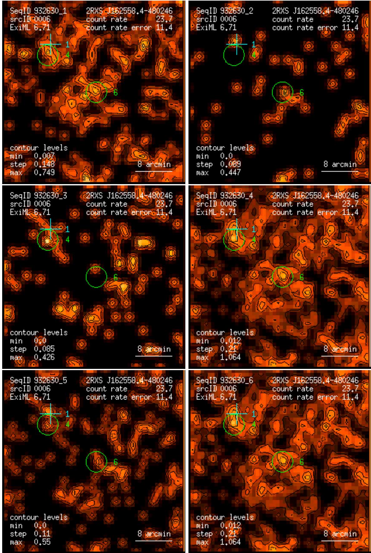
Figure 6: RASS 932630: detection 0006: band rate images, Gaussian filter: (1) PSPC channels 11 – 41, (2) 52 – 90, (3) 91 – 201, (4) 11 – 235, (5) 52 – 201, (6) 11 – 201. Broad band rates in counts/ks. Band rate contour levels in counts/ks/arcmin 2 .
