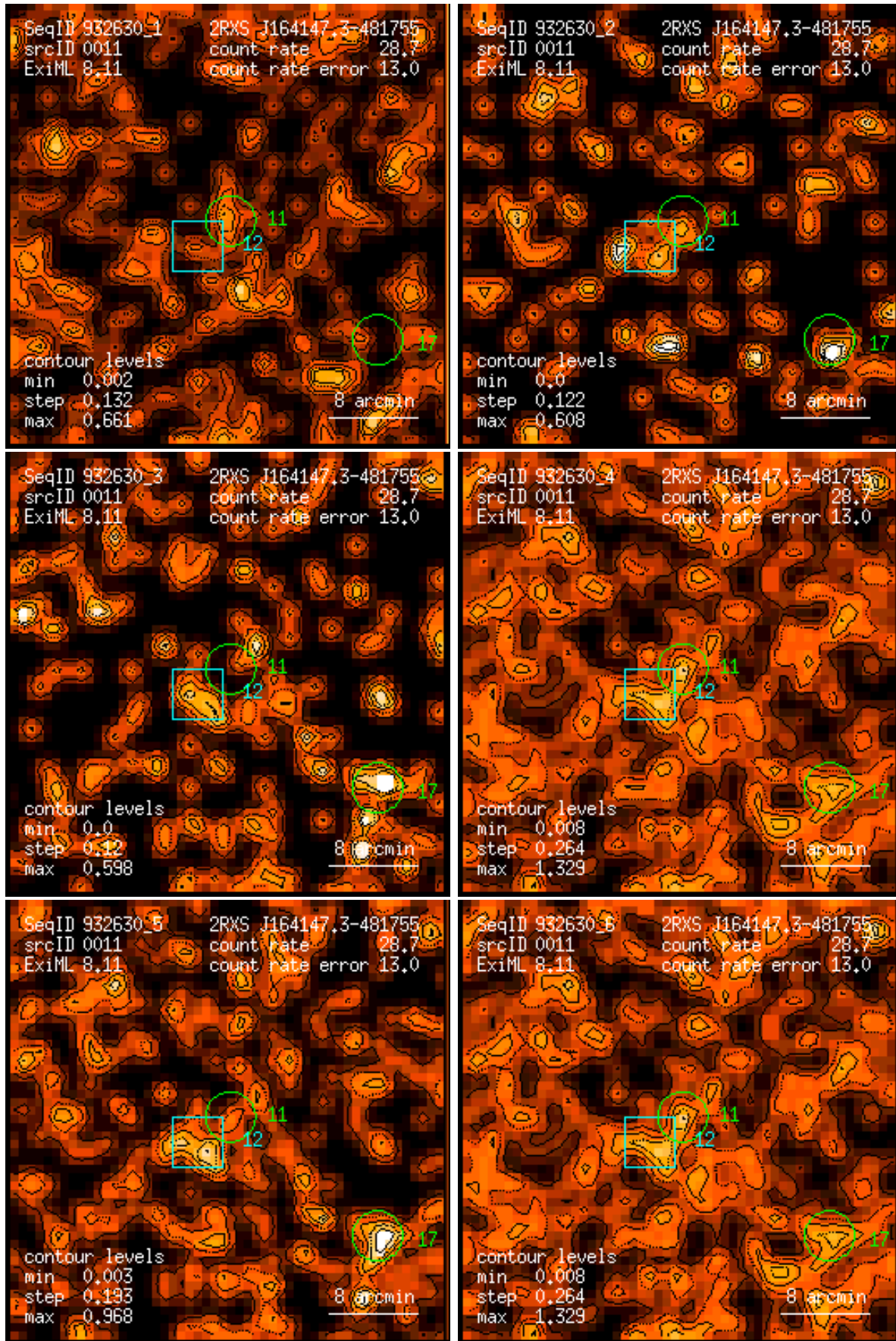
Figure 11: RASS 932630: detection 0011: band rate images, Gaussian filter: (1) PSPC channels 11 – 41, (2) 52 – 90, (3) 91 – 201, (4) 11 – 235, (5) 52 – 201, (6) 11 – 201. Broad band rates in counts/ks. Band rate contour levels in counts/ks/arcmin 2 .
