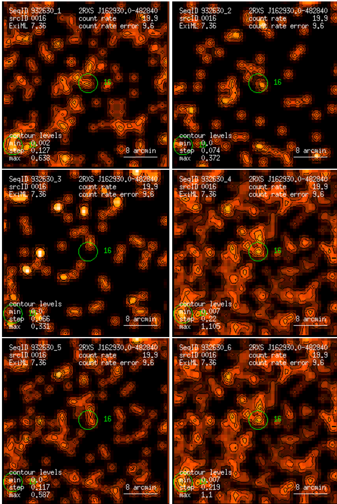
Figure 16: RASS 932630: detection 0016: band rate images, Gaussian filter: (1) PSPC channels 11 – 41, (2) 52 – 90, (3) 91 – 201, (4) 11 – 235, (5) 52 – 201, (6) 11 – 201. Broad band rates in counts/ks. Band rate contour levels in counts/ks/arcmin 2 .
