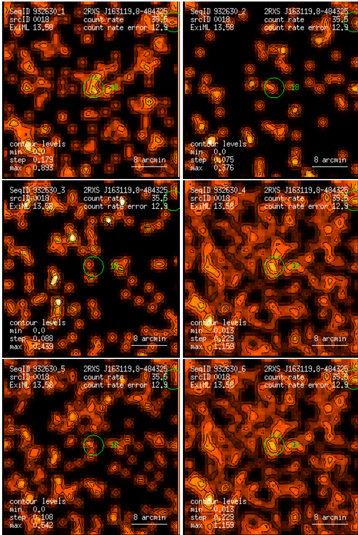
Figure 18: RASS 932630: detection 0018: band rate images, Gaussian filter: (1) PSPC channels 11 – 41, (2) 52 – 90, (3) 91 – 201, (4) 11 – 235, (5) 52 – 201, (6) 11 – 201. Broad band rates in counts/ks. Band rate contour levels in counts/ks/arcmin 2 .
