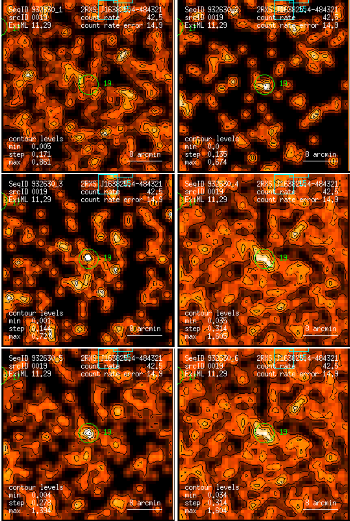
Figure 19: RASS 932630: detection 0019: band rate images, Gaussian filter: (1) PSPC channels 11 – 41, (2) 52 – 90, (3) 91 – 201, (4) 11 – 235, (5) 52 – 201, (6) 11 – 201. Broad band rates in counts/ks. Band rate contour levels in counts/ks/arcmin 2 .
