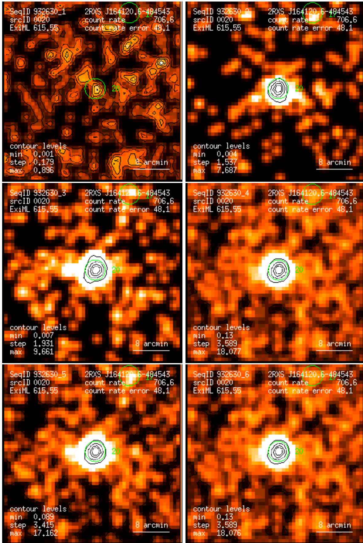
Figure 20: RASS 932630: detection 0020: band rate images, Gaussian filter: (1) PSPC channels 11 – 41, (2) 52 – 90, (3) 91 – 201, (4) 11 – 235, (5) 52 – 201, (6) 11 – 201. Broad band rates in counts/ks. Band rate contour levels in counts/ks/arcmin 2 .
