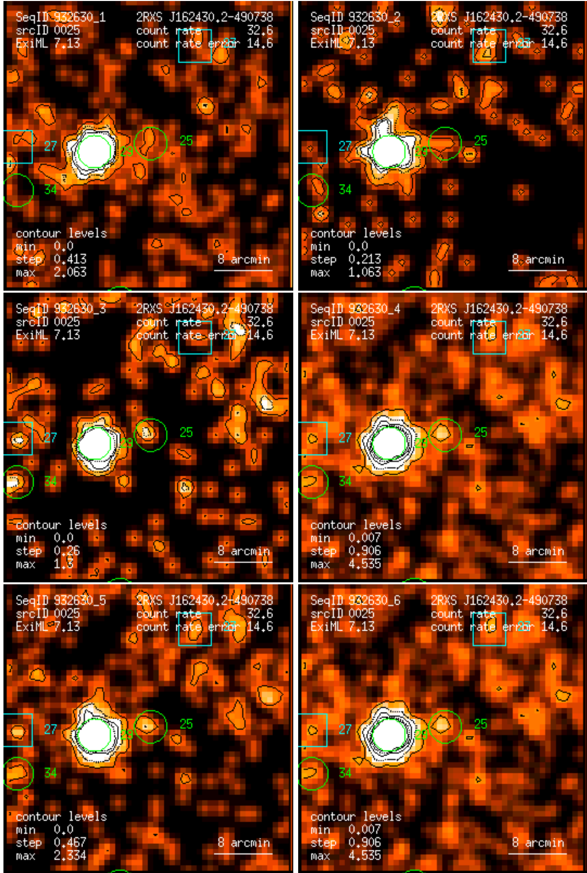
Figure 25: RASS 932630: detection 0025: band rate images, Gaussian filter: (1) PSPC channels 11 – 41, (2) 52 – 90, (3) 91 – 201, (4) 11 – 235, (5) 52 – 201, (6) 11 – 201. Broad band rates in counts/ks. Band rate contour levels in counts/ks/arcmin 2 .
