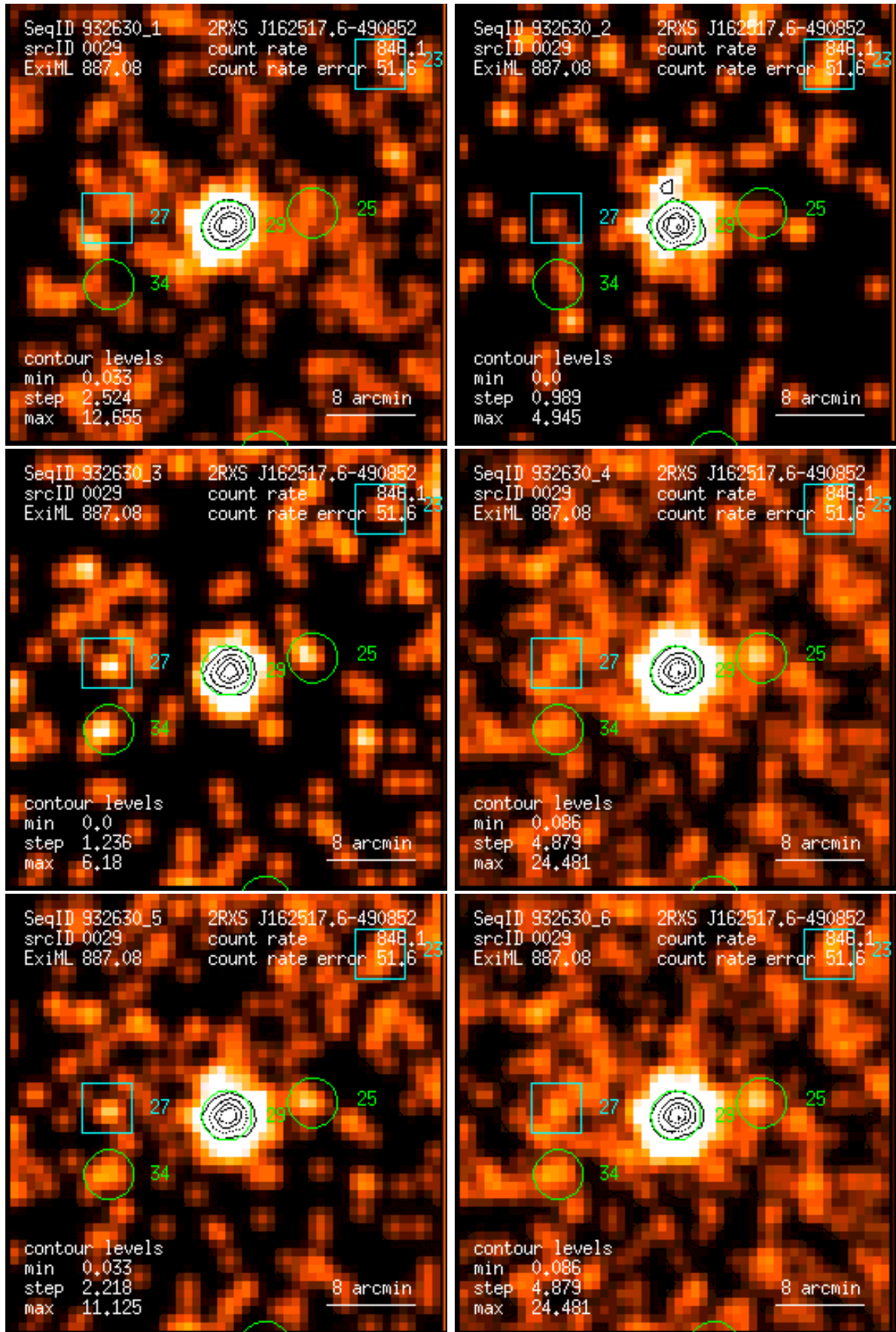
Figure 29: RASS 932630: detection 0029: band rate images, Gaussian filter: (1) PSPC channels 11 – 41, (2) 52 – 90, (3) 91 – 201, (4) 11 – 235, (5) 52 – 201, (6) 11 – 201. Broad band rates in counts/ks. Band rate contour levels in counts/ks/arcmin 2 .
