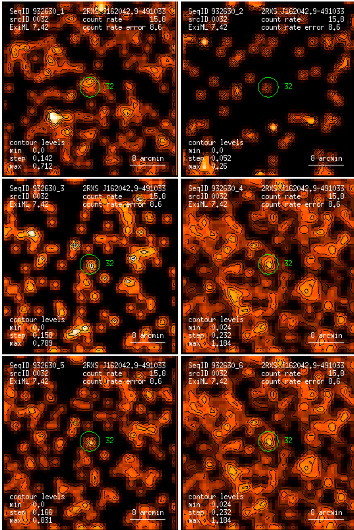
Figure 32: RASS 932630: detection 0032: band rate images, Gaussian filter: (1) PSPC channels 11 – 41, (2) 52 – 90, (3) 91 – 201, (4) 11 – 235, (5) 52 – 201, (6) 11 – 201. Broad band rates in counts/ks. Band rate contour levels in counts/ks/arcmin 2 .
