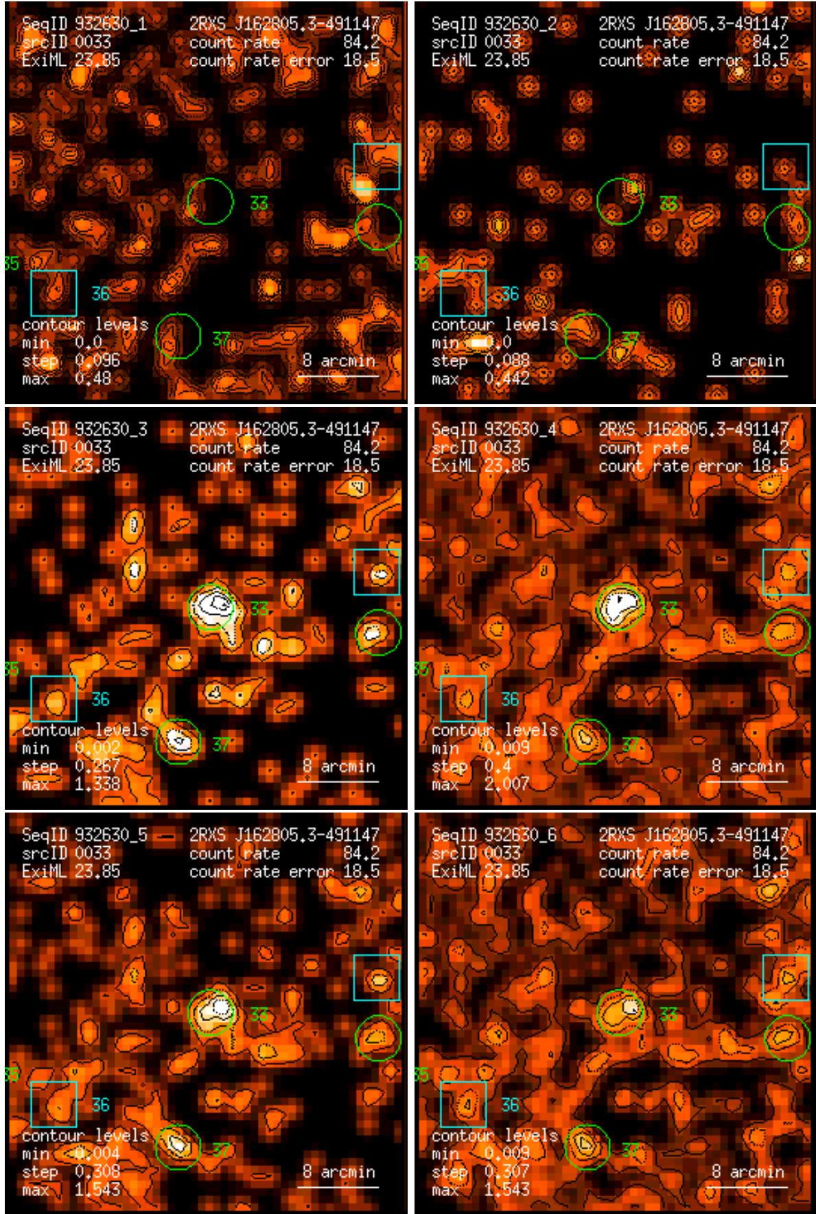
Figure 33: RASS 932630: detection 0033: band rate images, Gaussian filter: (1) PSPC channels 11 – 41, (2) 52 – 90, (3) 91 – 201, (4) 11 – 235, (5) 52 – 201, (6) 11 – 201. Broad band rates in counts/ks. Band rate contour levels in counts/ks/arcmin 2 .
