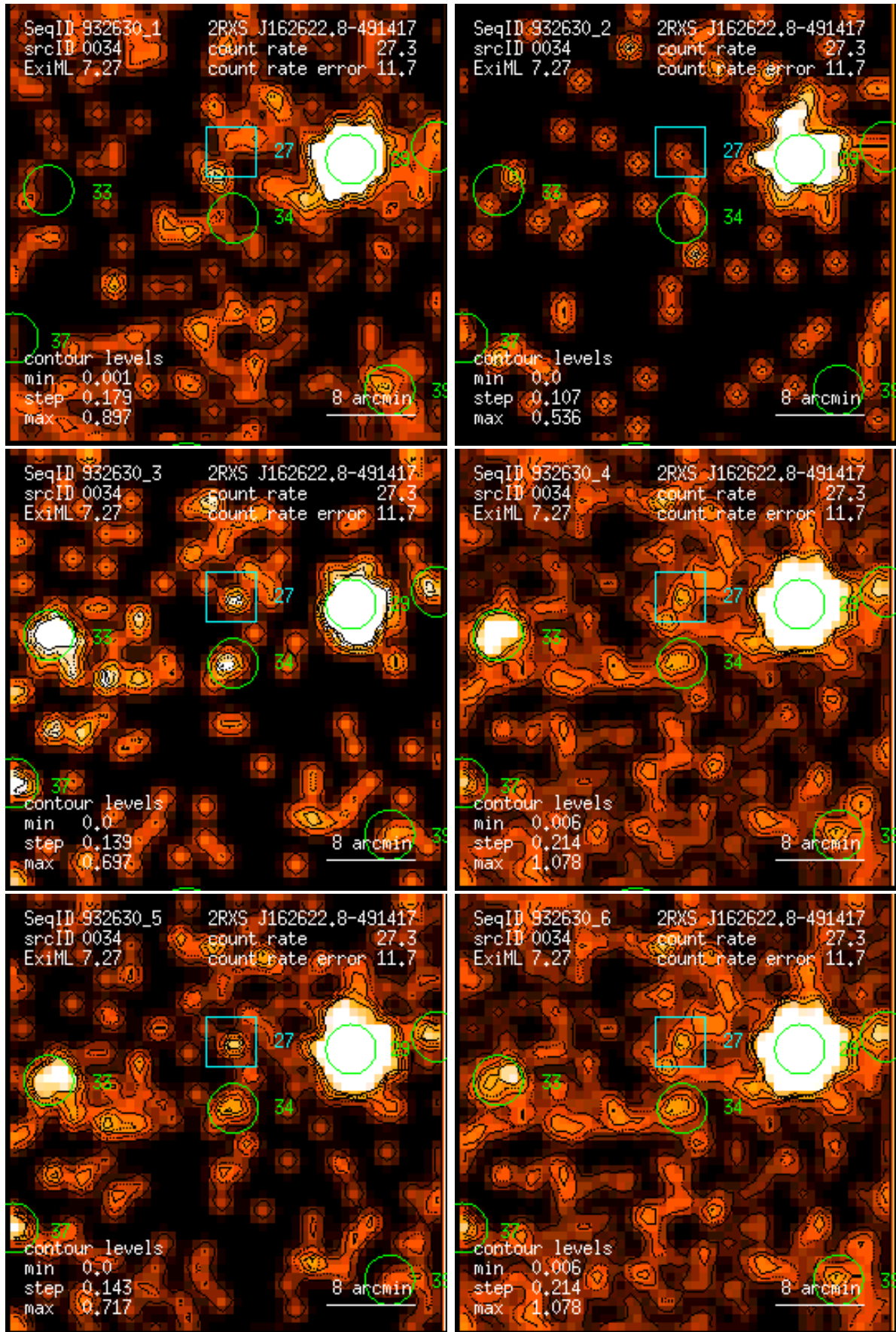
Figure 34: RASS 932630: detection 0034: band rate images, Gaussian filter: (1) PSPC channels 11 – 41, (2) 52 – 90, (3) 91 – 201, (4) 11 – 235, (5) 52 – 201, (6) 11 – 201. Broad band rates in counts/ks. Band rate contour levels in counts/ks/arcmin 2 .
