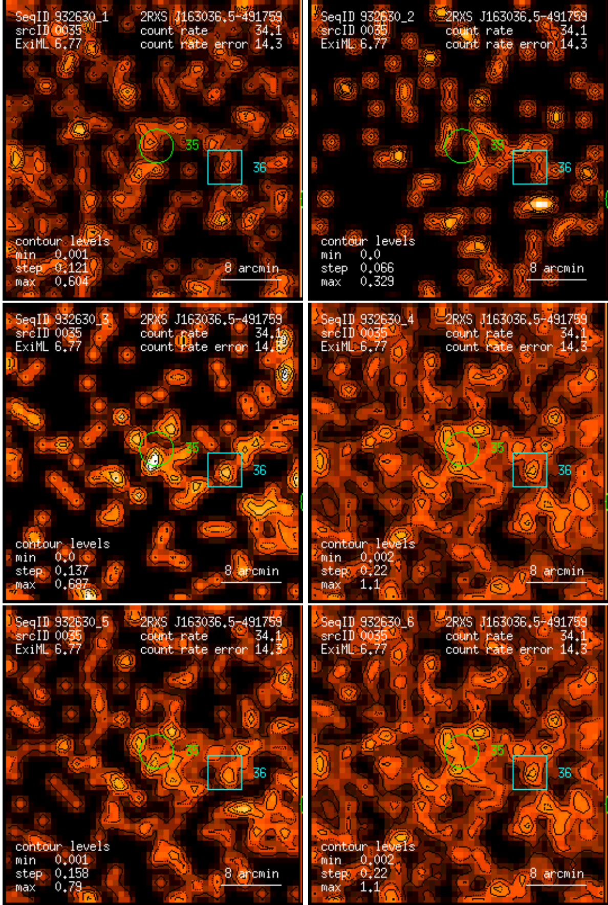
Figure 35: RASS 932630: detection 0035: band rate images, Gaussian filter: (1) PSPC channels 11 – 41, (2) 52 – 90, (3) 91 – 201, (4) 11 – 235, (5) 52 – 201, (6) 11 – 201. Broad band rates in counts/ks. Band rate contour levels in counts/ks/arcmin 2 .
