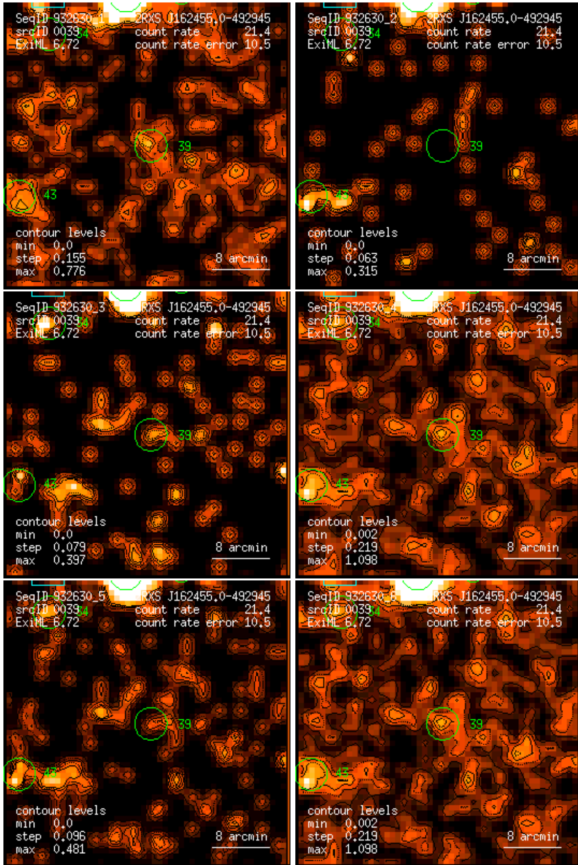
Figure 39: RASS 932630: detection 0039: band rate images, Gaussian filter: (1) PSPC channels 11 – 41, (2) 52 – 90, (3) 91 – 201, (4) 11 – 235, (5) 52 – 201, (6) 11 – 201. Broad band rates in counts/ks. Band rate contour levels in counts/ks/arcmin 2 .
