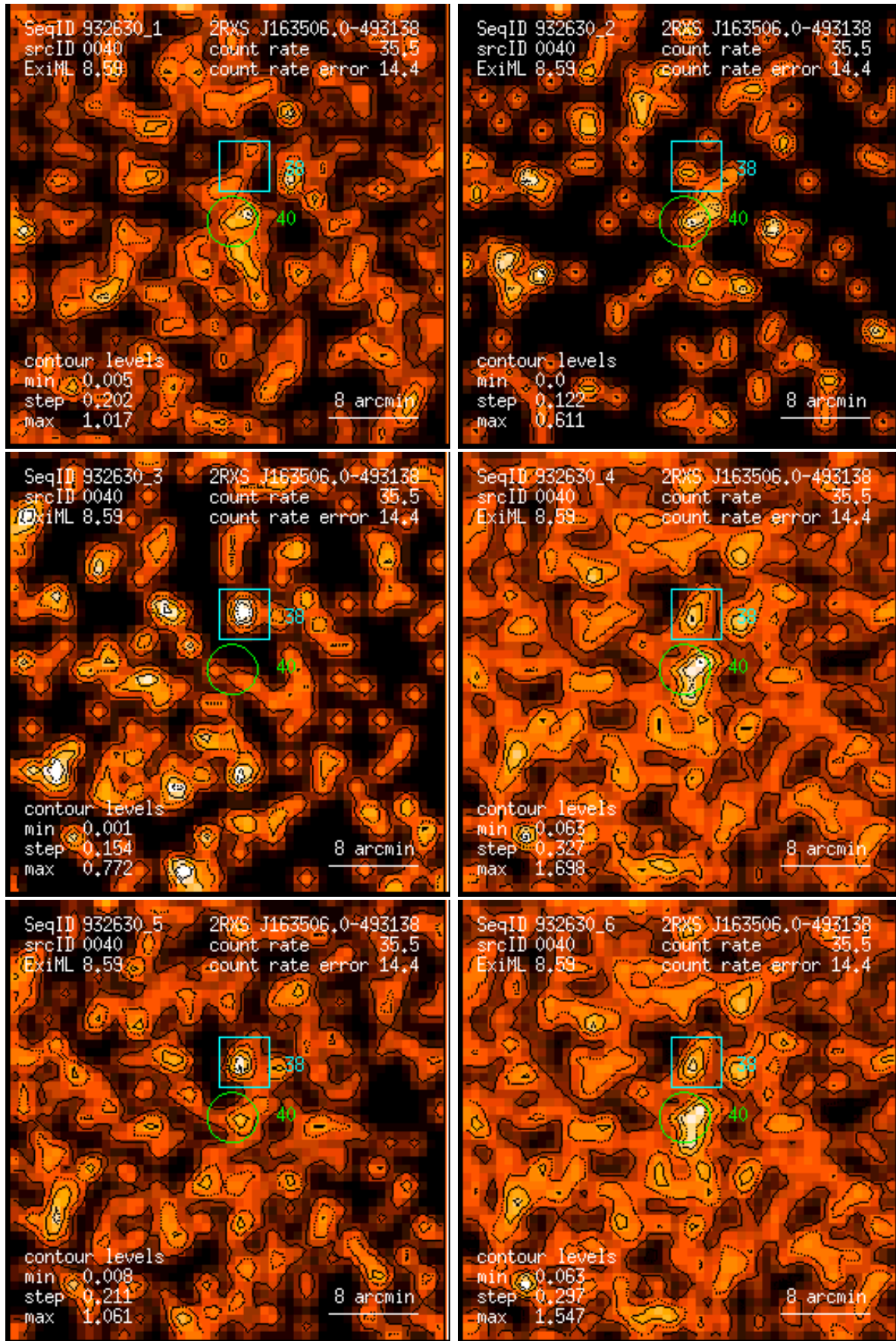
Figure 40: RASS 932630: detection 0040: band rate images, Gaussian filter: (1) PSPC channels 11 – 41, (2) 52 – 90, (3) 91 – 201, (4) 11 – 235, (5) 52 – 201, (6) 11 – 201. Broad band rates in counts/ks. Band rate contour levels in counts/ks/arcmin 2 .
