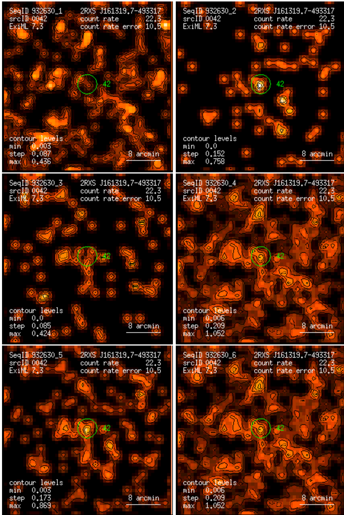
Figure 42: RASS 932630: detection 0042: band rate images, Gaussian filter: (1) PSPC channels 11 – 41, (2) 52 – 90, (3) 91 – 201, (4) 11 – 235, (5) 52 – 201, (6) 11 – 201. Broad band rates in counts/ks. Band rate contour levels in counts/ks/arcmin 2 .
