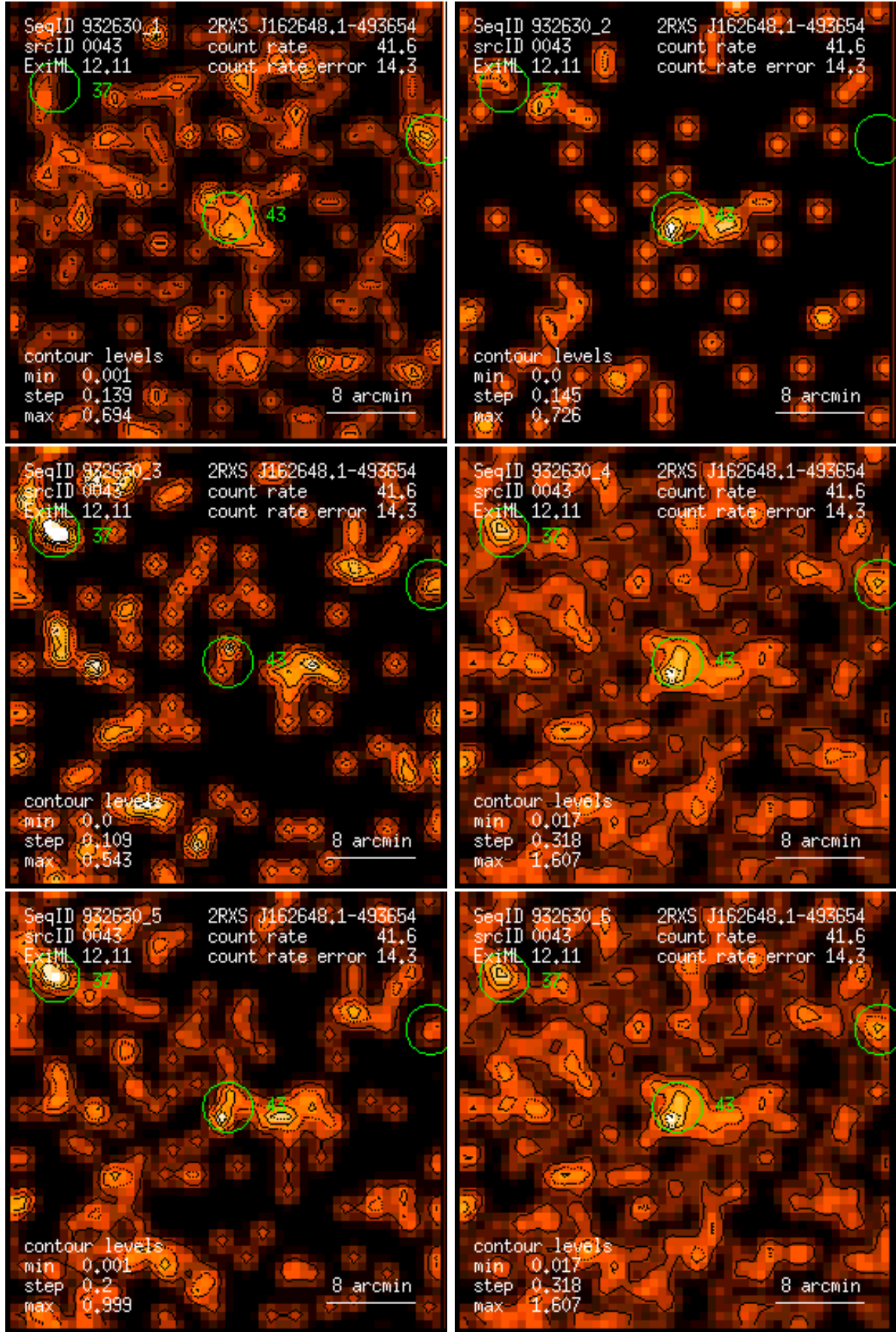
Figure 43: RASS 932630: detection 0043: band rate images, Gaussian filter: (1) PSPC channels 11 – 41, (2) 52 – 90, (3) 91 – 201, (4) 11 – 235, (5) 52 – 201, (6) 11 – 201. Broad band rates in counts/ks. Band rate contour levels in counts/ks/arcmin 2 .
