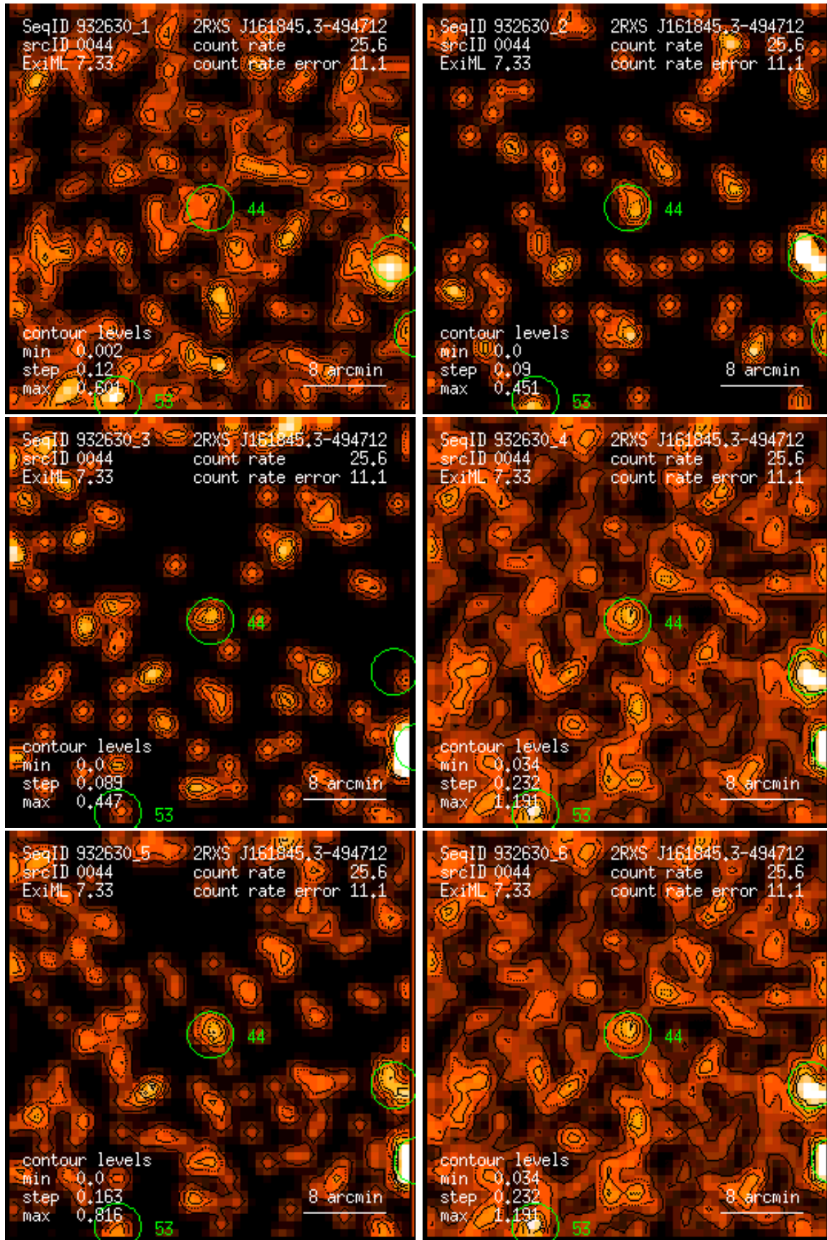
Figure 44: RASS 932630: detection 0044: band rate images, Gaussian filter: (1) PSPC channels 11 – 41, (2) 52 – 90, (3) 91 – 201, (4) 11 – 235, (5) 52 – 201, (6) 11 – 201. Broad band rates in counts/ks. Band rate contour levels in counts/ks/arcmin 2 .
