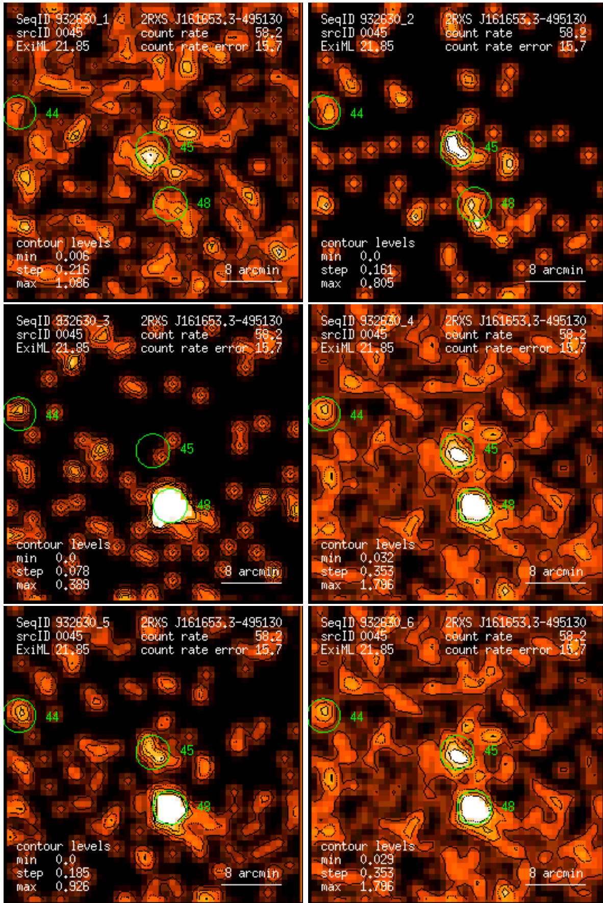
Figure 45: RASS 932630: detection 0045: band rate images, Gaussian filter: (1) PSPC channels 11 – 41, (2) 52 – 90, (3) 91 – 201, (4) 11 – 235, (5) 52 – 201, (6) 11 – 201. Broad band rates in counts/ks. Band rate contour levels in counts/ks/arcmin 2 .
