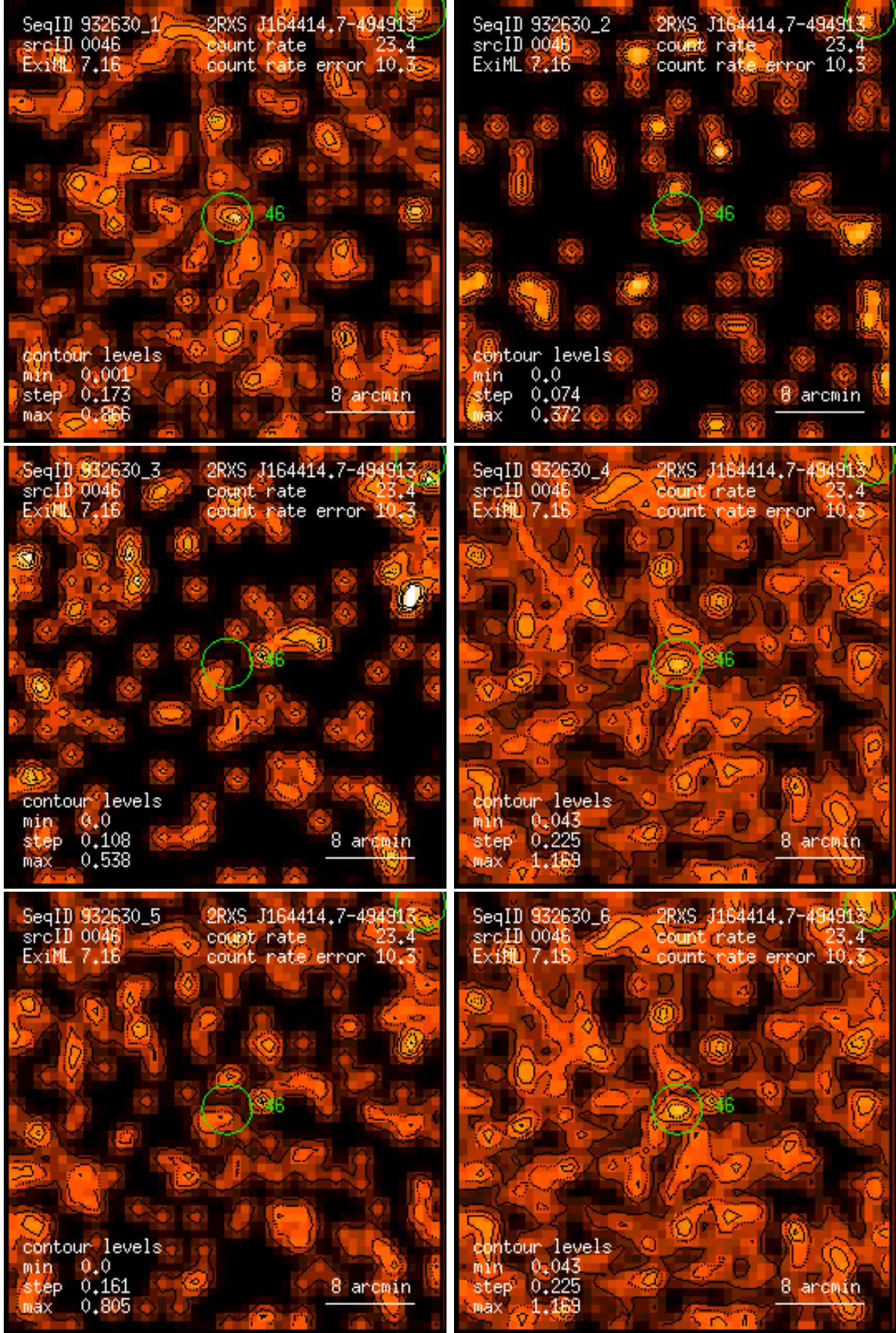
Figure 46: RASS 932630: detection 0046: band rate images, Gaussian filter: (1) PSPC channels 11 – 41, (2) 52 – 90, (3) 91 – 201, (4) 11 – 235, (5) 52 – 201, (6) 11 – 201. Broad band rates in counts/ks. Band rate contour levels in counts/ks/arcmin 2 .
