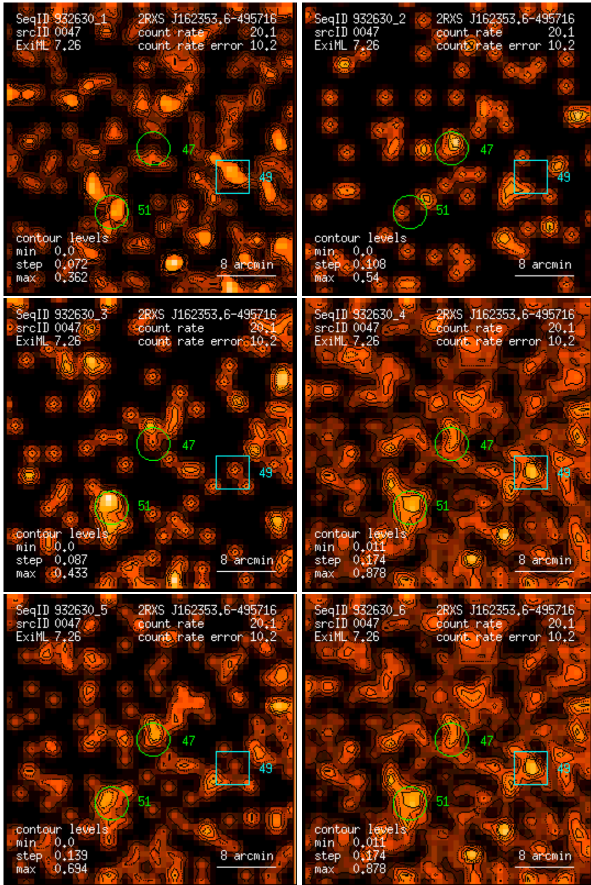
Figure 47: RASS 932630: detection 0047: band rate images, Gaussian filter: (1) PSPC channels 11 – 41, (2) 52 – 90, (3) 91 – 201, (4) 11 – 235, (5) 52 – 201, (6) 11 – 201. Broad band rates in counts/ks. Band rate contour levels in counts/ks/arcmin 2 .
