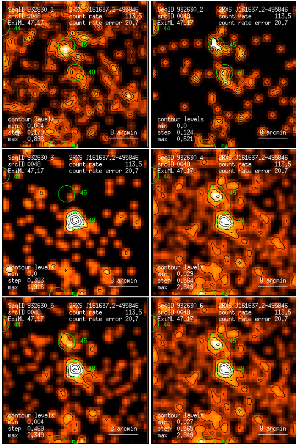
Figure 48: RASS 932630: detection 0048: band rate images, Gaussian filter: (1) PSPC channels 11 – 41, (2) 52 – 90, (3) 91 – 201, (4) 11 – 235, (5) 52 – 201, (6) 11 – 201. Broad band rates in counts/ks. Band rate contour levels in counts/ks/arcmin 2 .
