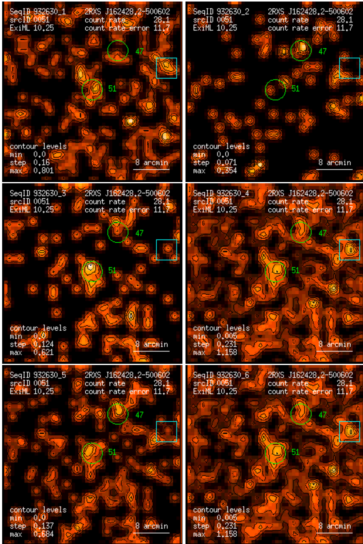
Figure 51: RASS 932630: detection 0051: band rate images, Gaussian filter: (1) PSPC channels 11 – 41, (2) 52 – 90, (3) 91 – 201, (4) 11 – 235, (5) 52 – 201, (6) 11 – 201. Broad band rates in counts/ks. Band rate contour levels in counts/ks/arcmin 2 .
