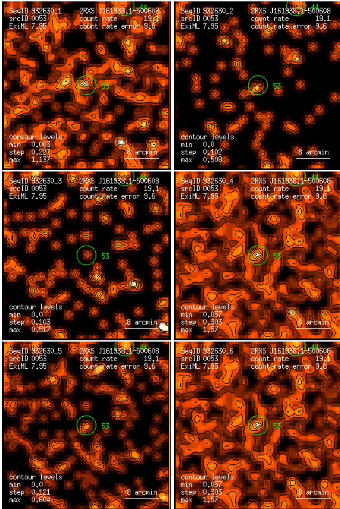
Figure 53: RASS 932630: detection 0053: band rate images, Gaussian filter: (1) PSPC channels 11 – 41, (2) 52 – 90, (3) 91 – 201, (4) 11 – 235, (5) 52 – 201, (6) 11 – 201. Broad band rates in counts/ks. Band rate contour levels in counts/ks/arcmin 2 .
