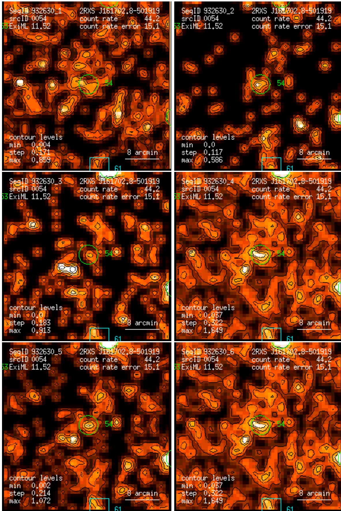
Figure 54: RASS 932630: detection 0054: band rate images, Gaussian filter: (1) PSPC channels 11 – 41, (2) 52 – 90, (3) 91 – 201, (4) 11 – 235, (5) 52 – 201, (6) 11 – 201. Broad band rates in counts/ks. Band rate contour levels in counts/ks/arcmin 2 .
