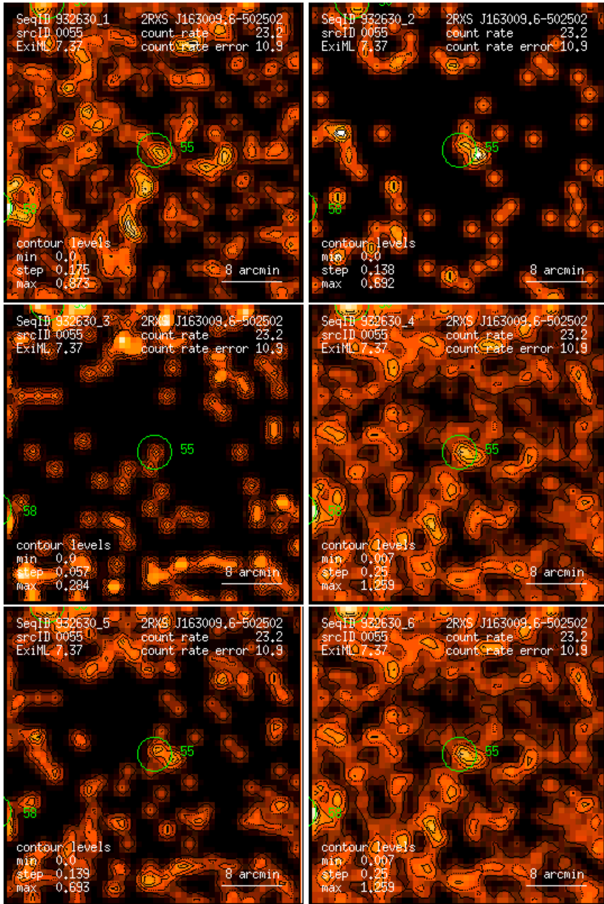
Figure 55: RASS 932630: detection 0055: band rate images, Gaussian filter: (1) PSPC channels 11 – 41, (2) 52 – 90, (3) 91 – 201, (4) 11 – 235, (5) 52 – 201, (6) 11 – 201. Broad band rates in counts/ks. Band rate contour levels in counts/ks/arcmin 2 .
